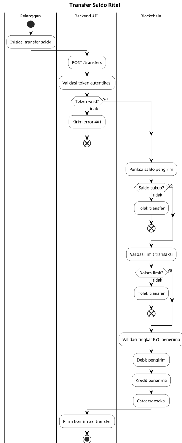
Gambar 3.17. Activity diagram transfer saldo ritel
