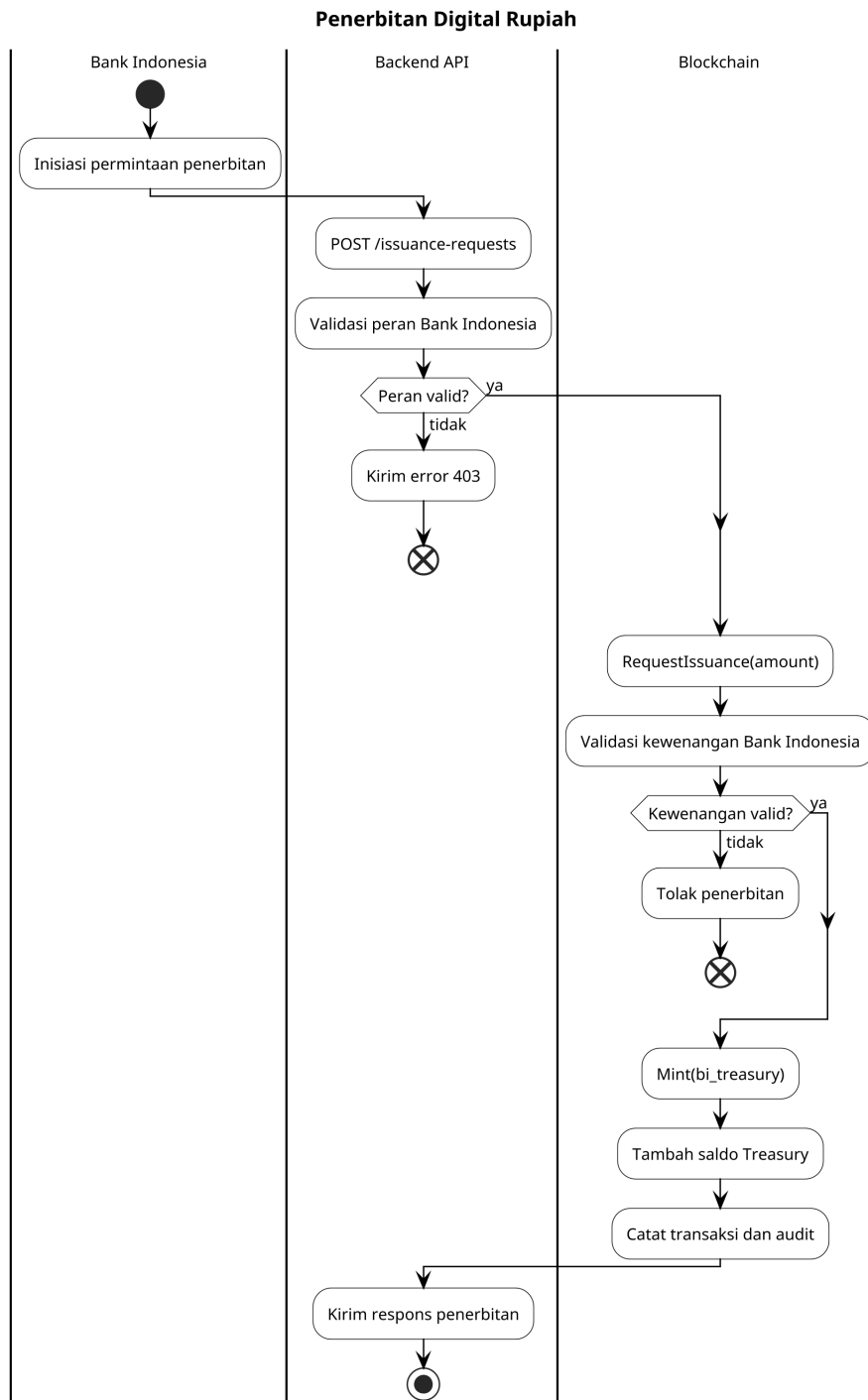
Gambar 3.15. Activity diagram penerbitan Digital Rupiah
