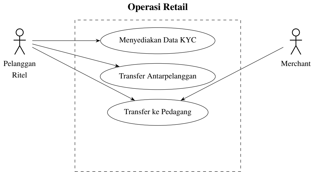
Gambar 3.28. Diagram use case operasi ritel
