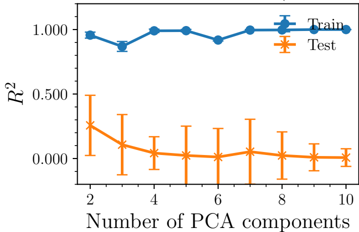
GPR R^2 vs. PCA components (1_2, Mean \pm SD)
