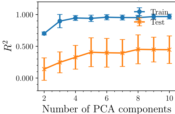
GPR R^2 vs. PCA components (full, Mean \pm SD)
