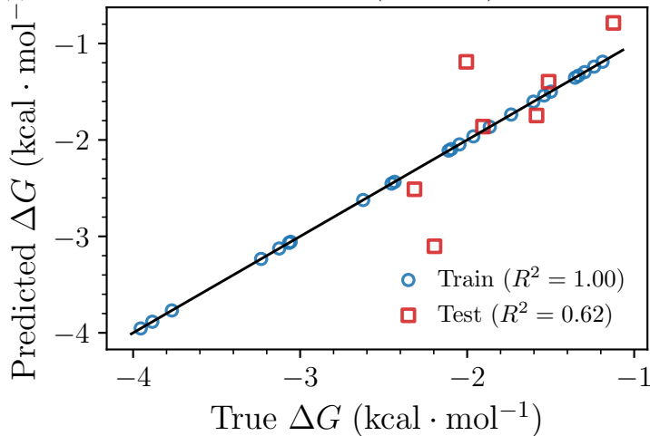
PCA10 (seed=2)
