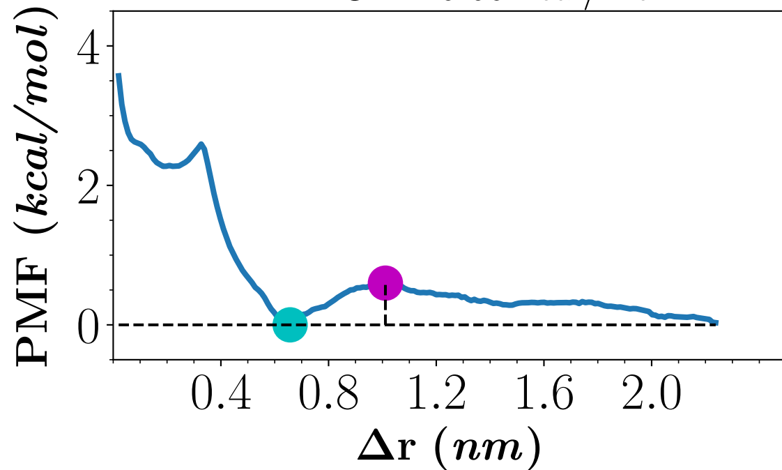
H19: \Delta G^\ddagger = 1.45 kcal/mol
