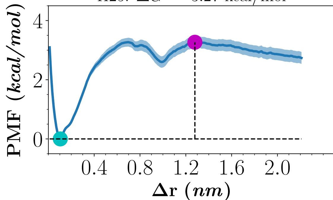
H25: \Delta G^\ddagger = 3.27 kcal/mol
