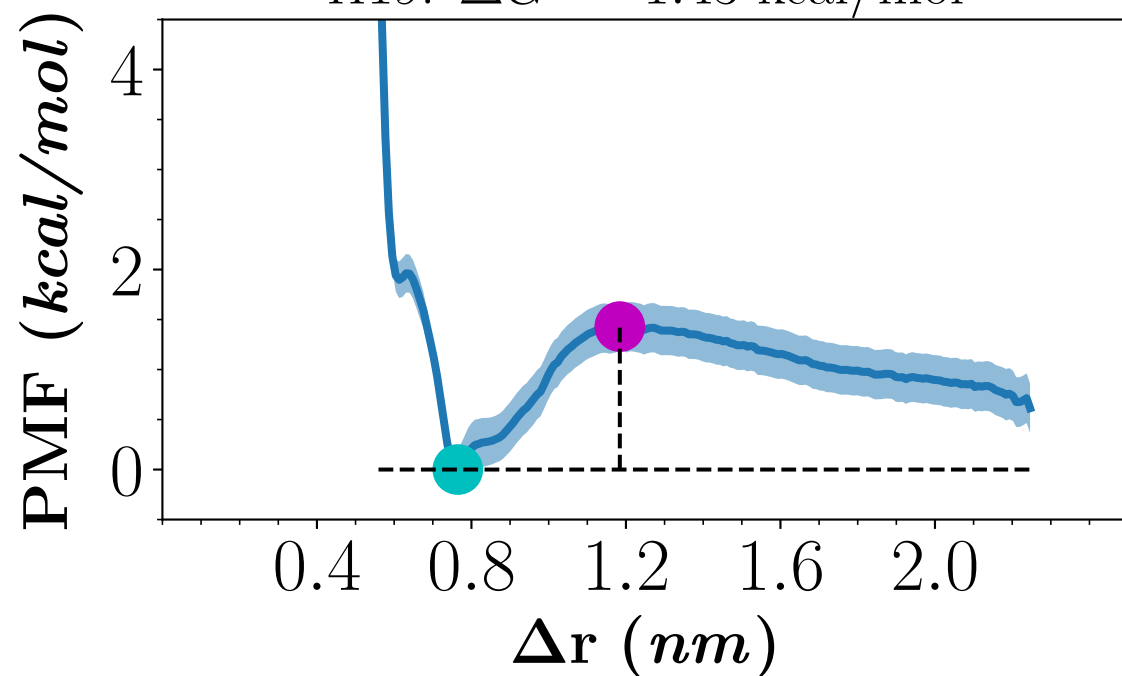
H19: \Delta G^\ddagger = 1.43 kcal/mol
