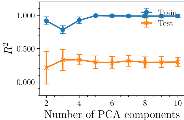
GPR R^2 vs. PCA components (3_4, Mean \pm SD)
