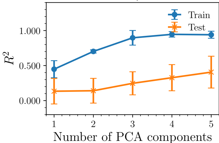
GPR R^2 vs. PCA (full, Mean \pm SD)
