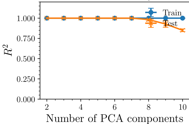
GPR R^2 vs. PCA components (1_2, Mean \pm SD)
