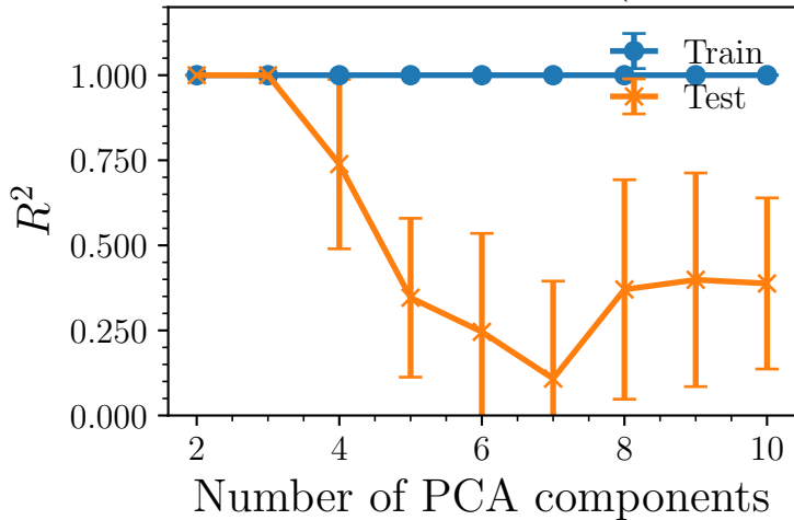
GPR R^2 vs. PCA components (1_4, Mean \pm SD)
