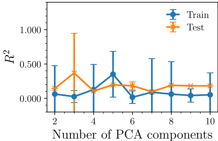
GPR R^2 vs. PCA components (1_5, Mean \pm SD)
