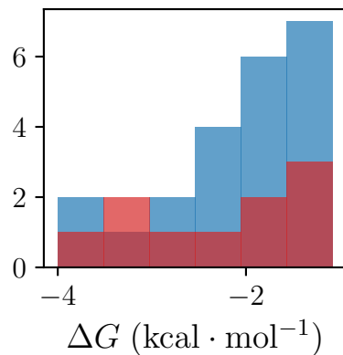
Fold 3
