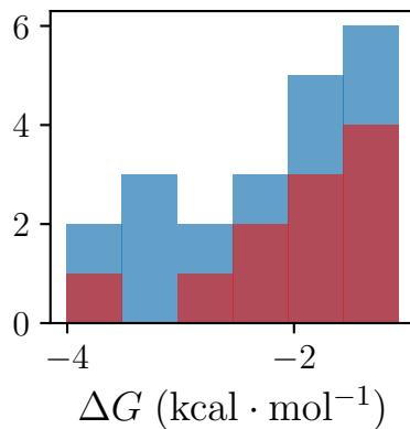
Fold 2
