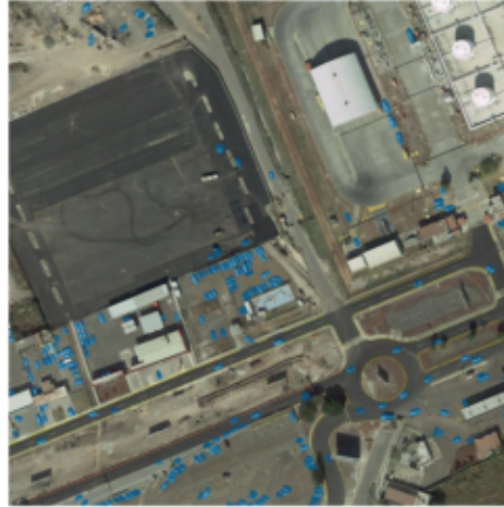
Reference union
