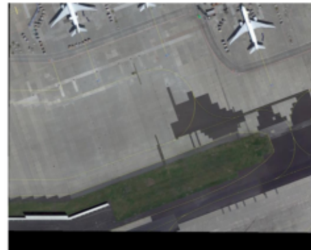
SAM1
