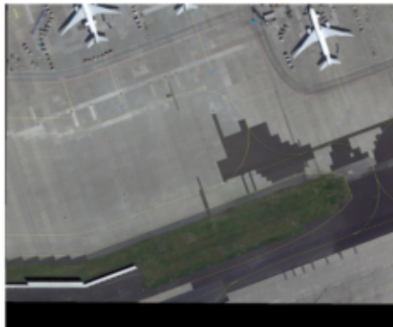
Reference union
