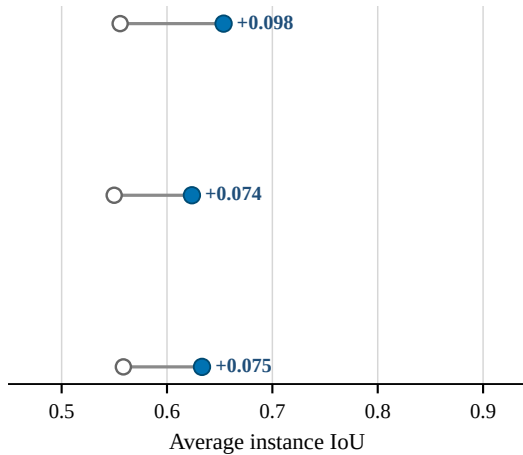
(b) iSAID Small Vehicle
