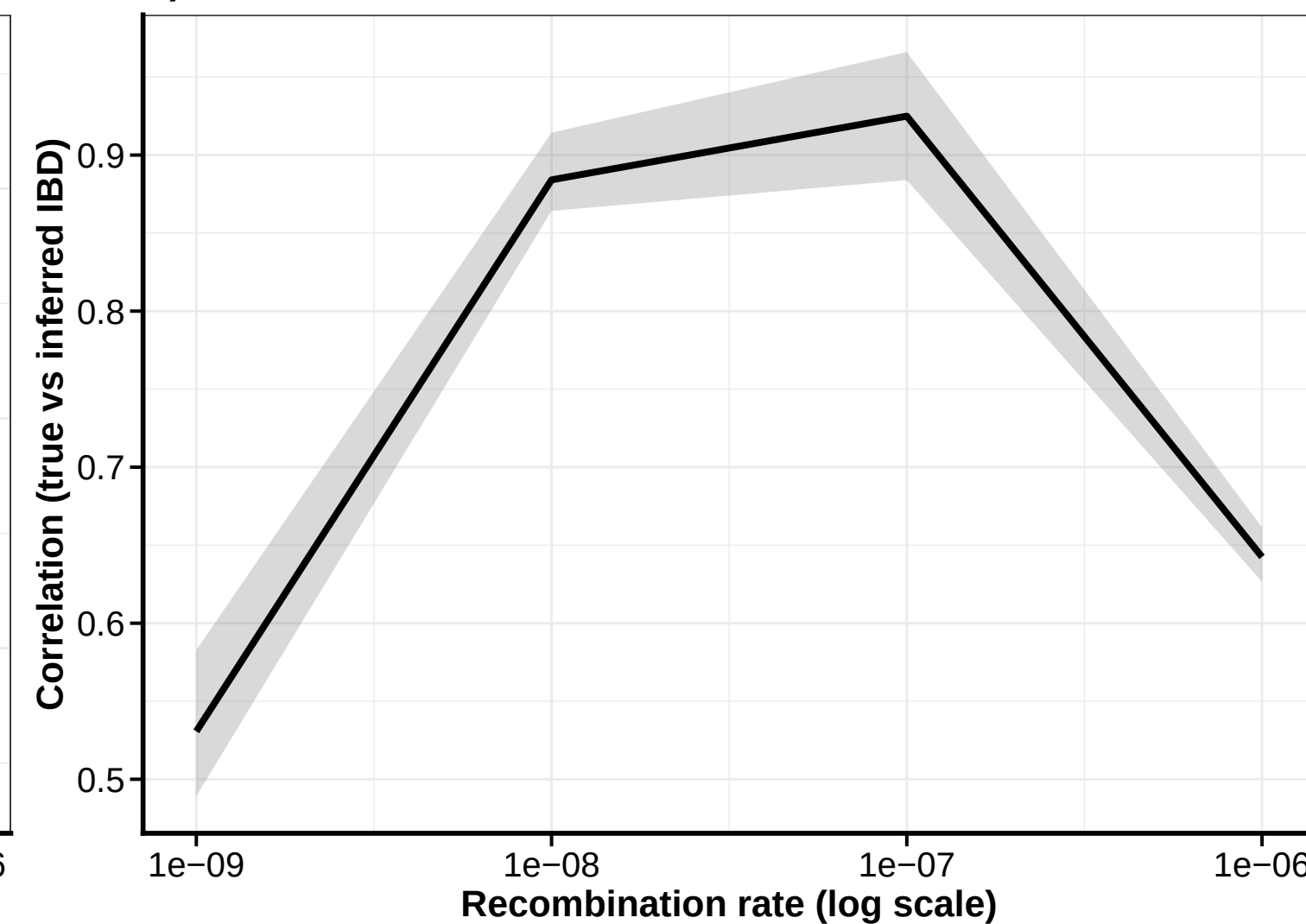
D) Correlation between true and inferred IBD
