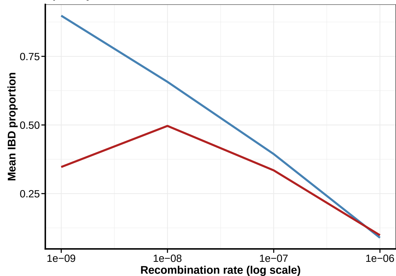
C) Decay of true and inferred IBD across recombination rates
