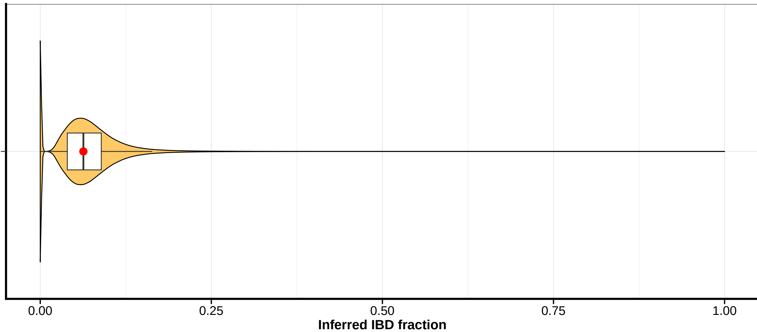
B) Inferred IBD Fraction (hmmIBD)
