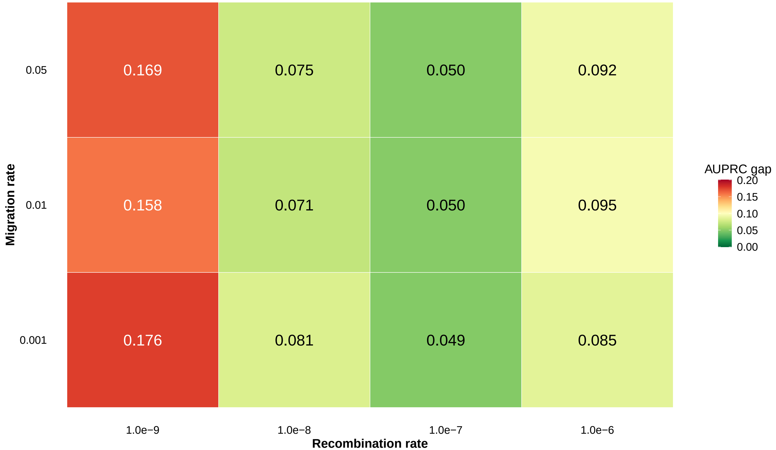
IBD advantage over next-best method (AUPRC gap = IBD - max(IBS, Phylo), G ≤ 25)
