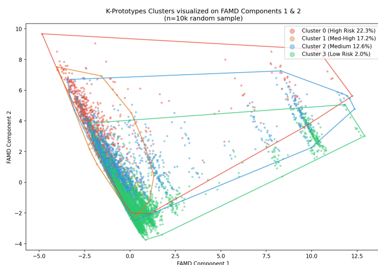
Figure 10: K-Prototype Clusters
