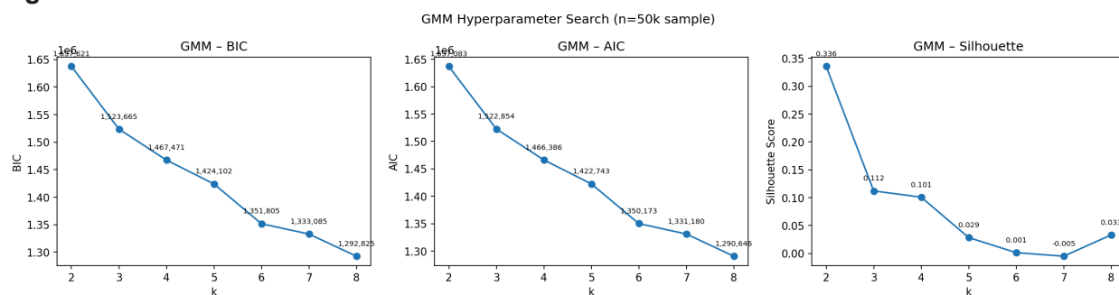
Figure 9: GMM Evaluation
