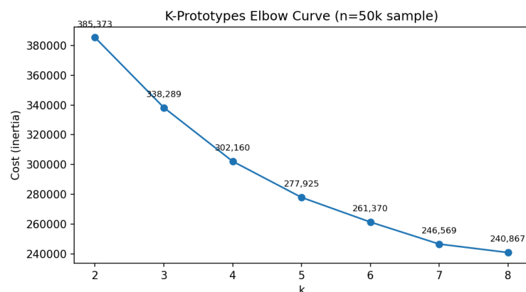
Figure 8: K-Prototypes Metrics
