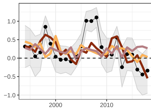
B. Leave-one-out predictions
