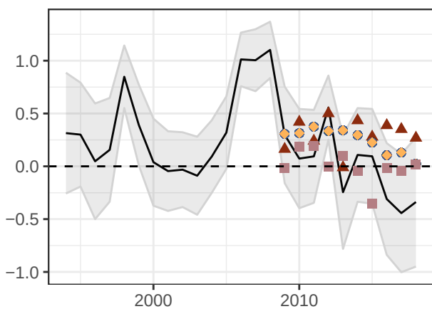
A. One-year-ahead predictions
