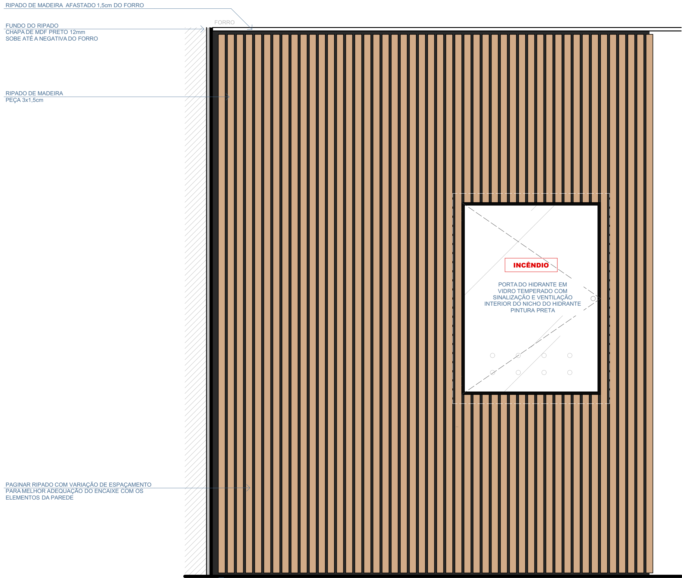
VISTA FRONTAL
