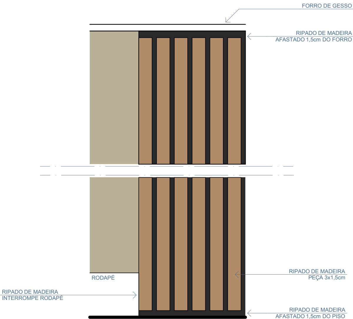
VISTA FRONTAL
