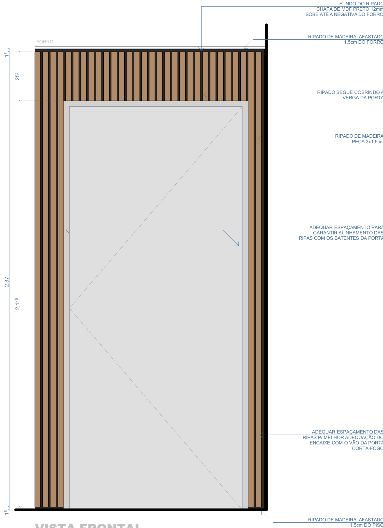
VISTA FRONTAL
