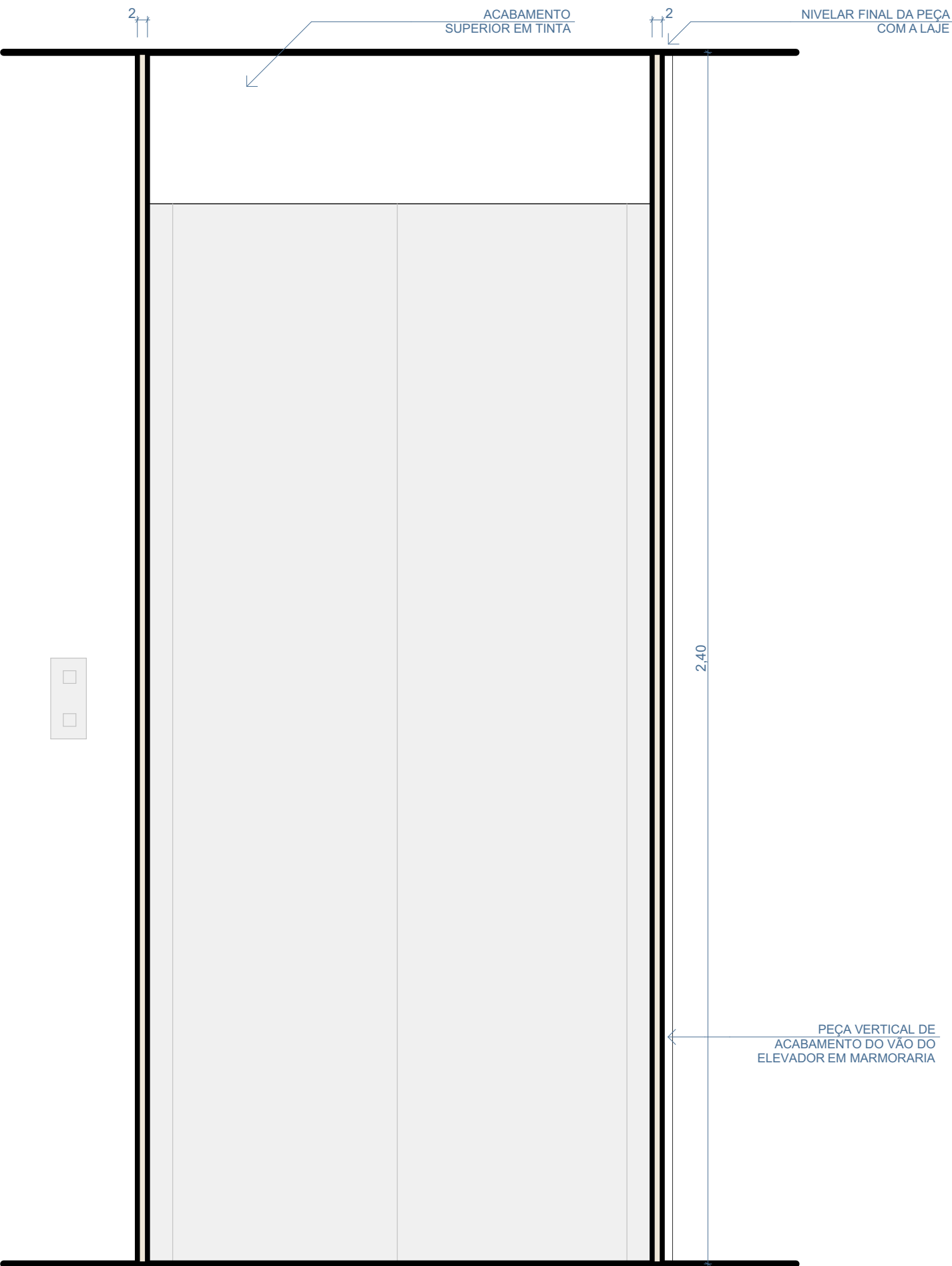
VISTA FRONTAL
