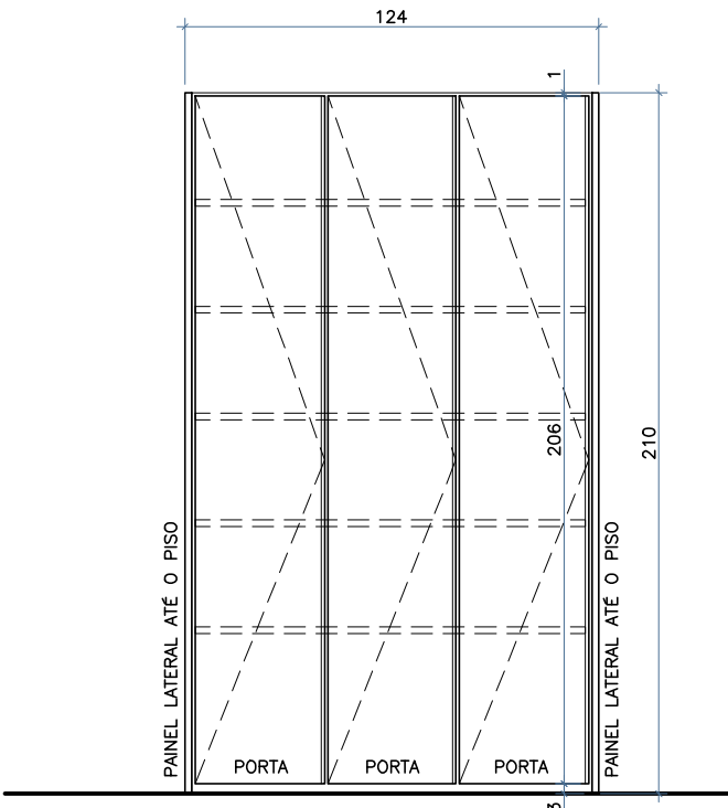
VISTA FRONTAL
