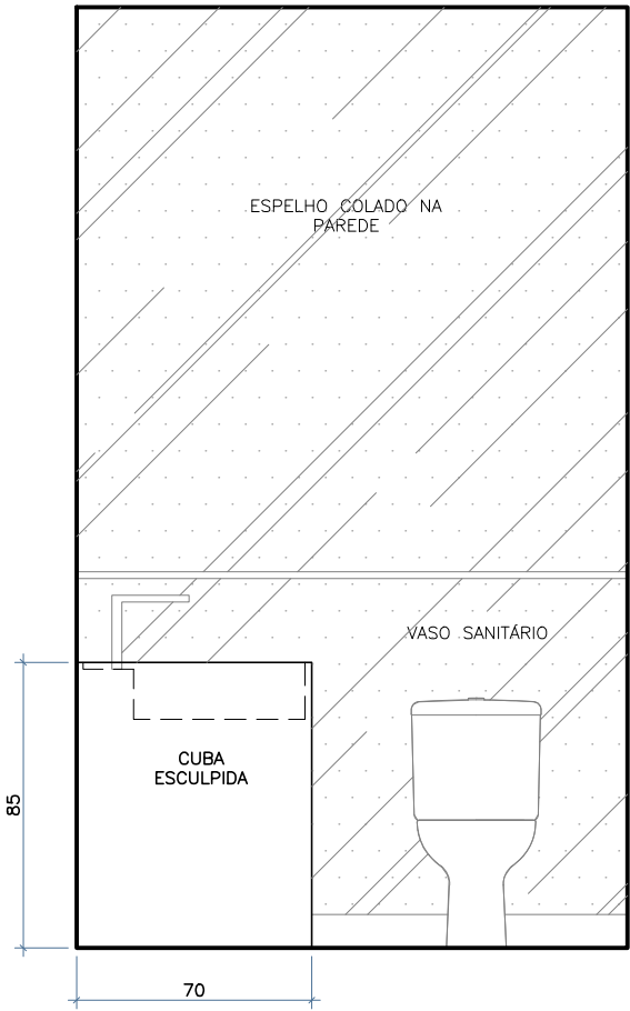
VISTA FRONTAL
