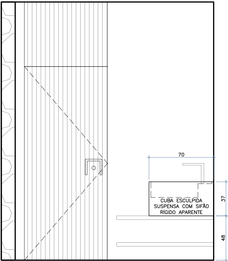
VISTA FRONTAL
