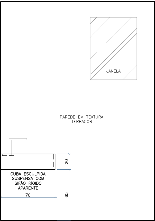
VISTA FRONTAL
