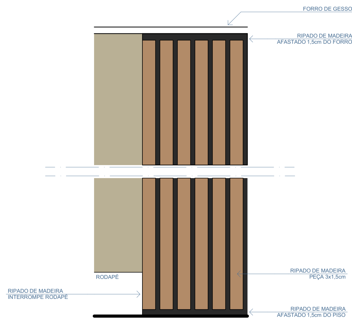
VISTA FRONTAL
