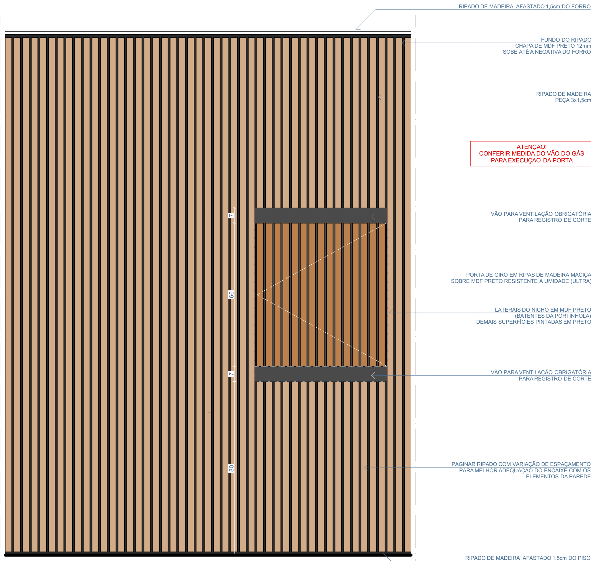
VISTA FRONTAL
