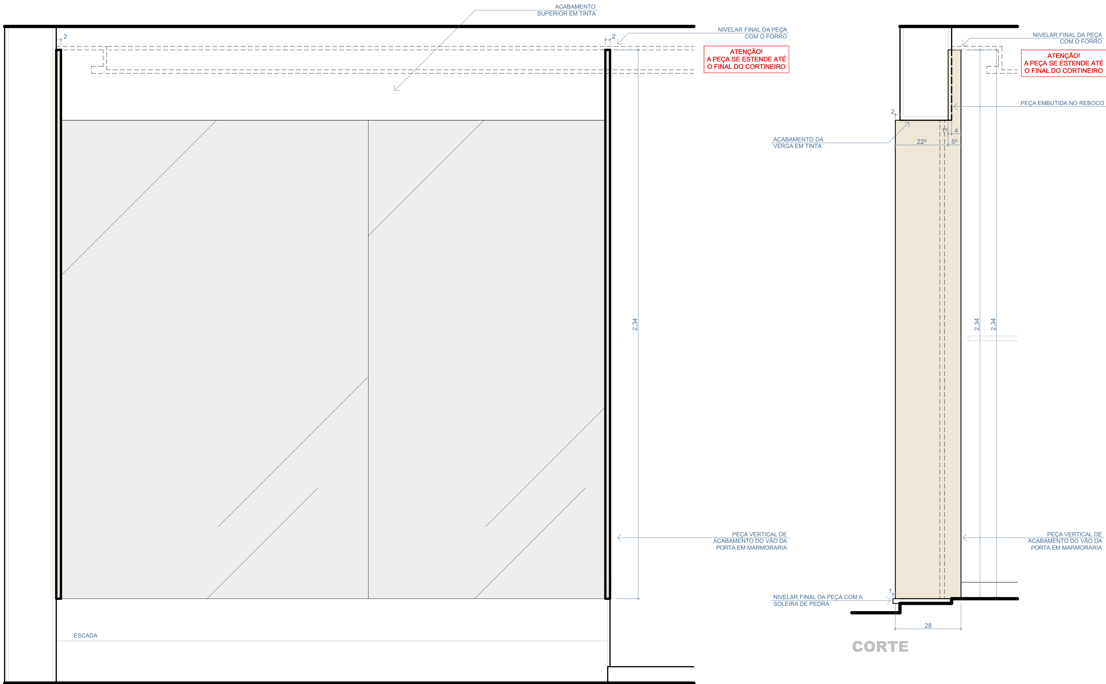
VISTA FRONTAL
