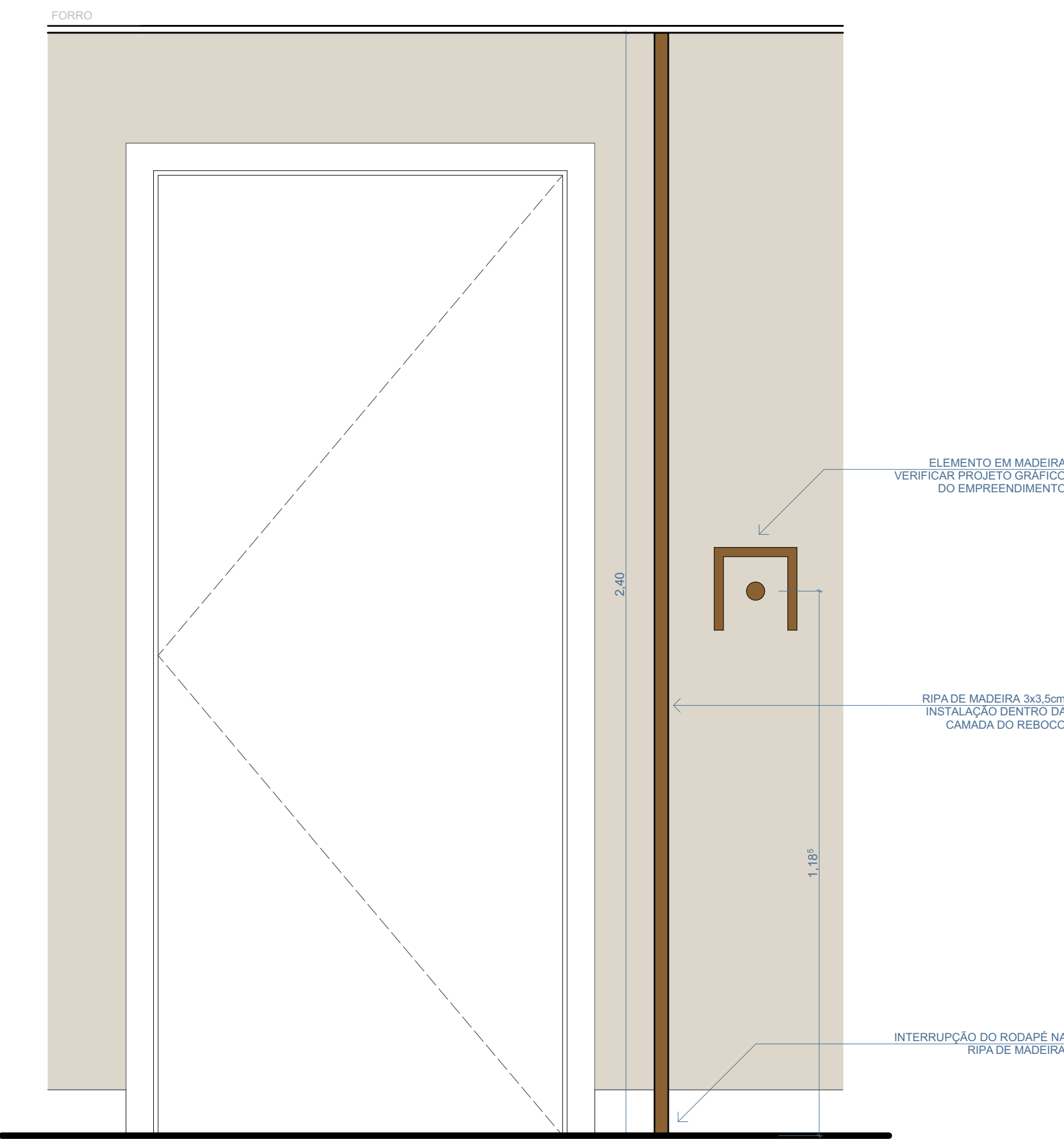
VISTA FRONTAL
