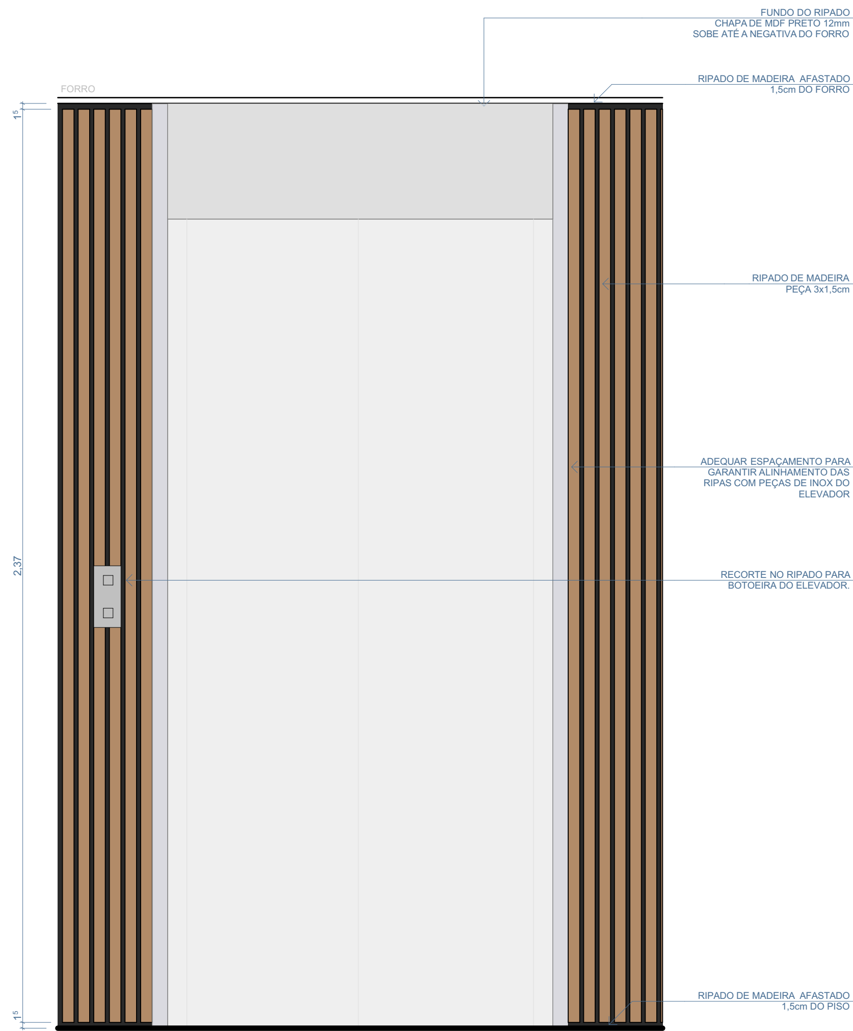
VISTA FRONTAL
