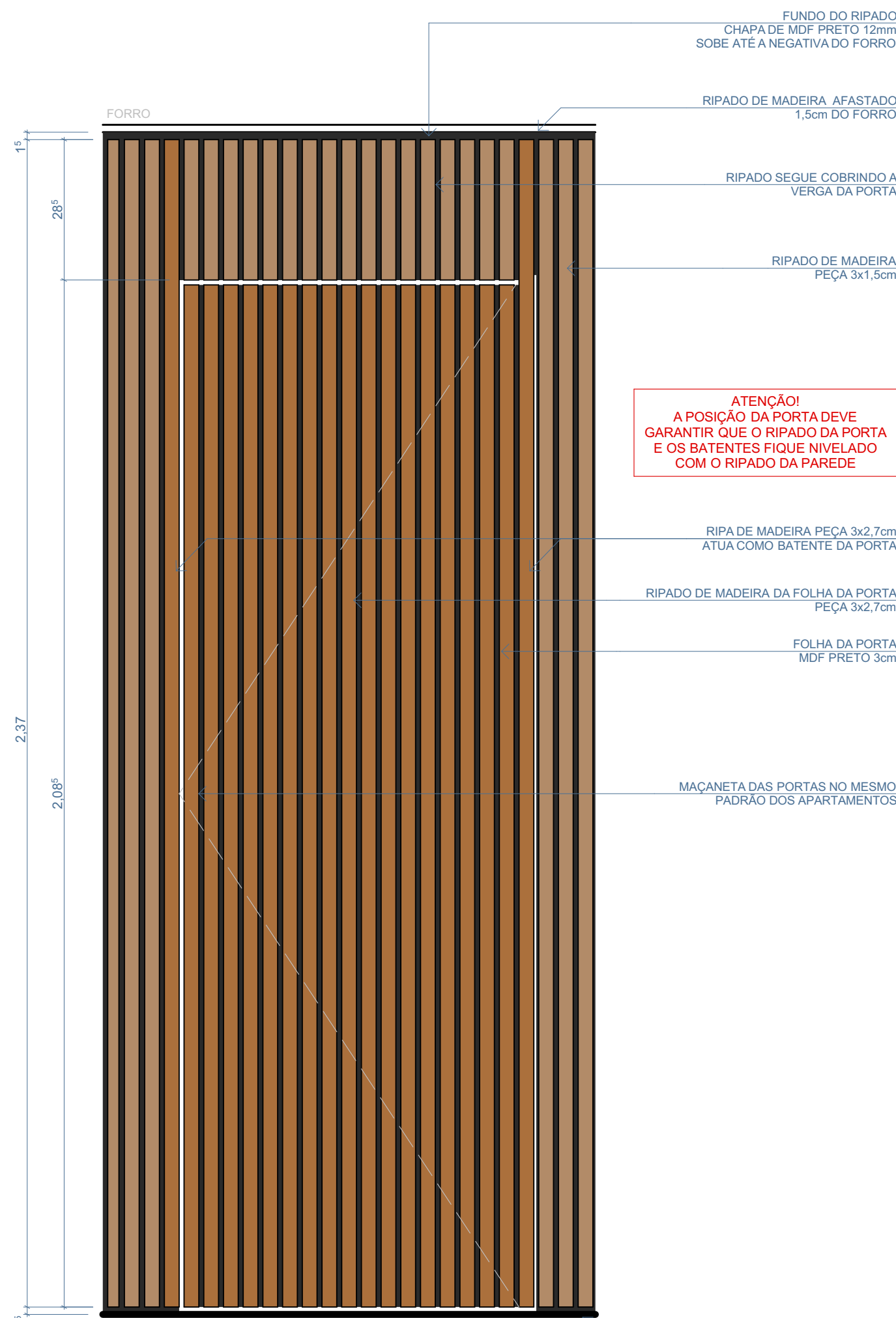
VISTA FRONTAL
