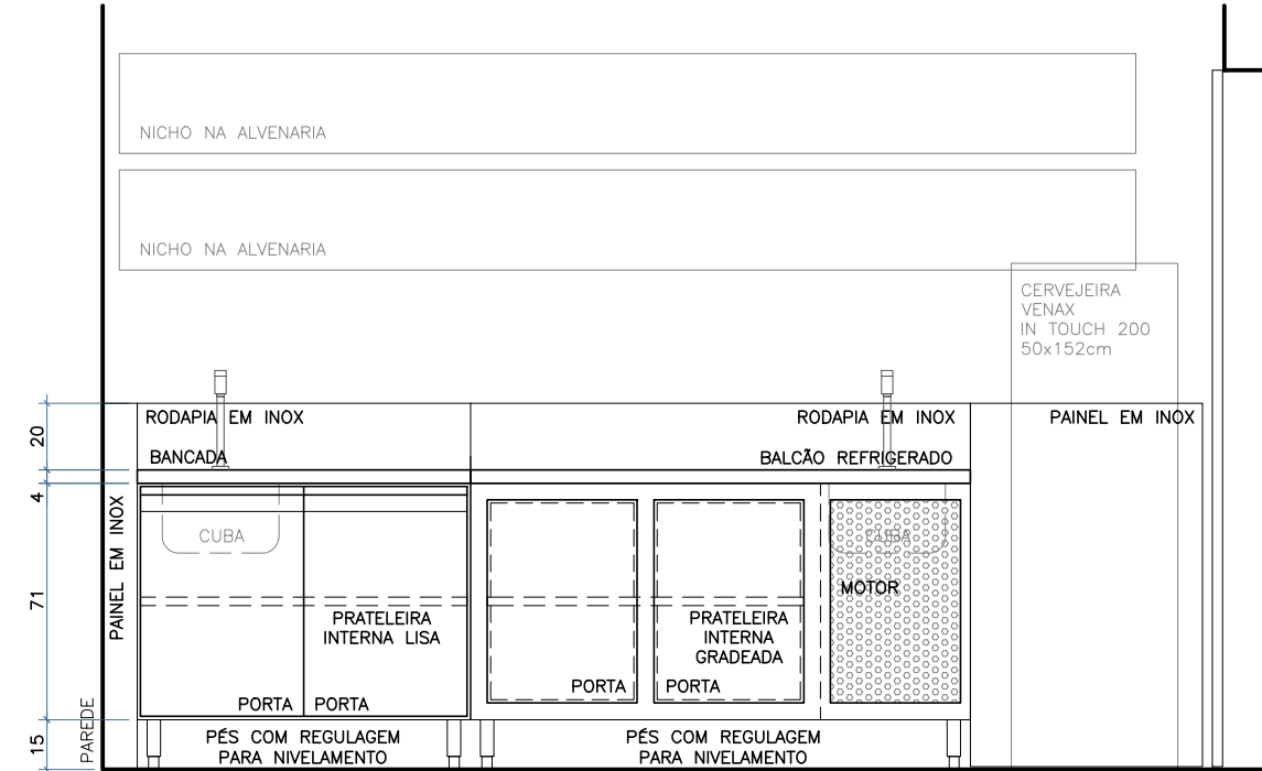
VISTA FRONTAL
