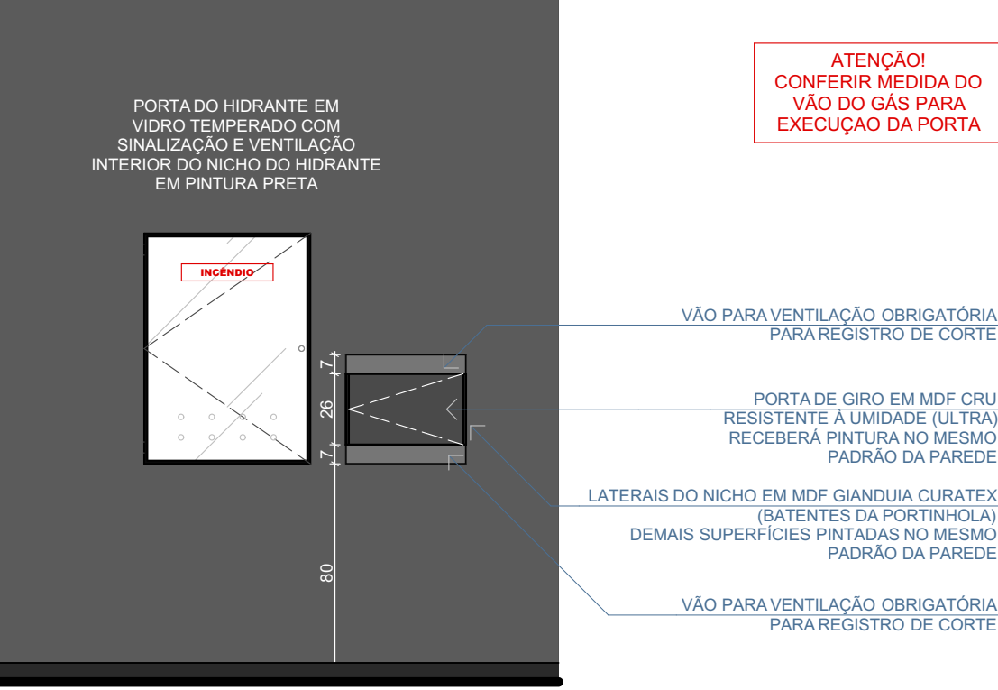
VISTA FRONTAL
