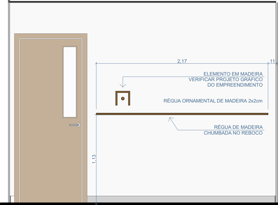
VISTA FRONTAL
