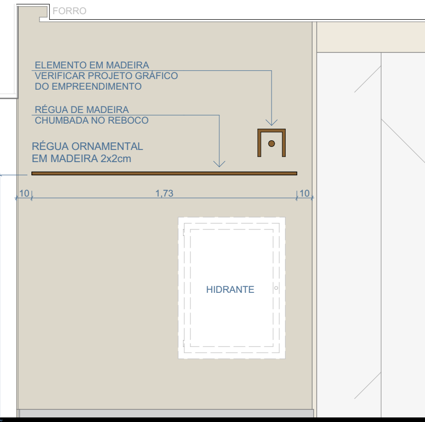
VISTA FRONTAL
