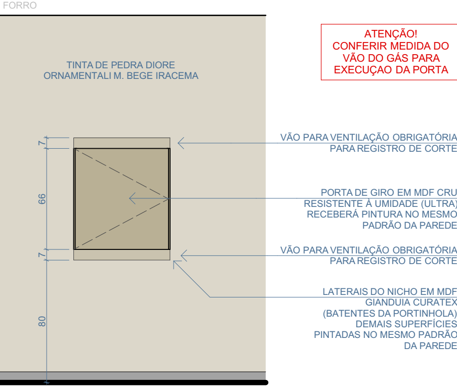
VISTA FRONTAL
