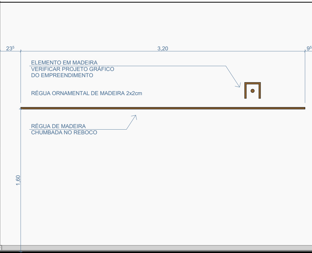
VISTA FRONTAL
