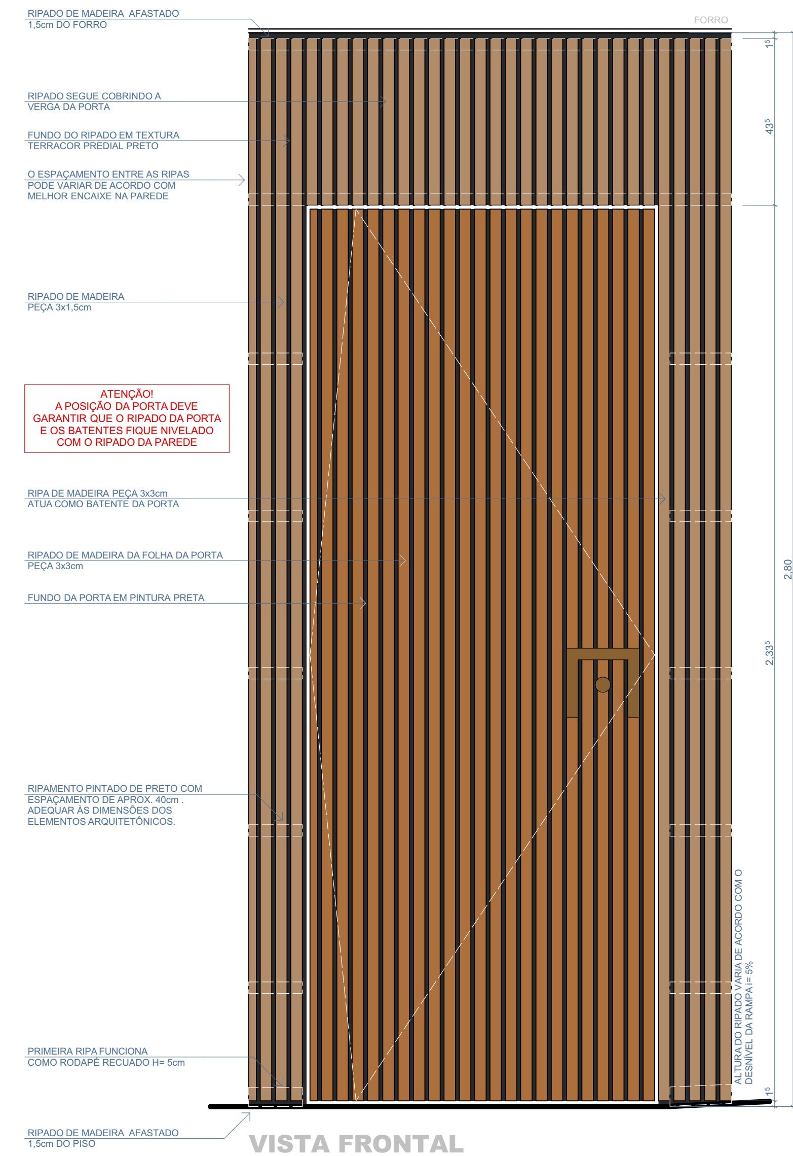
VISTA FRONTAL
