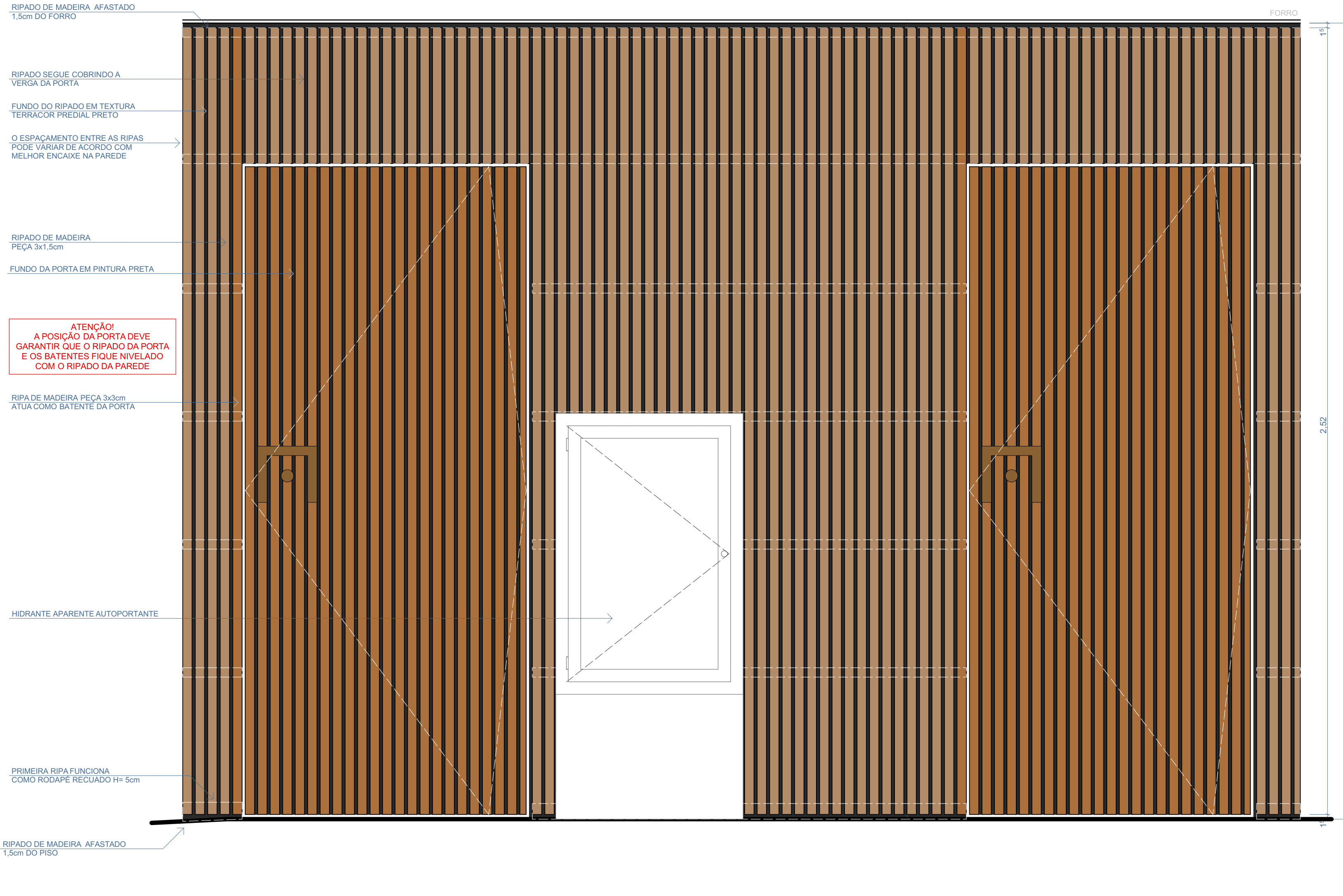
VISTA FRONTAL
