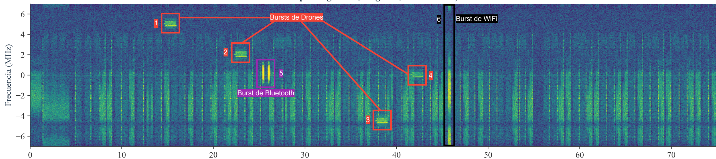
Espectrograma (Target=6, SNR=-14dB)
