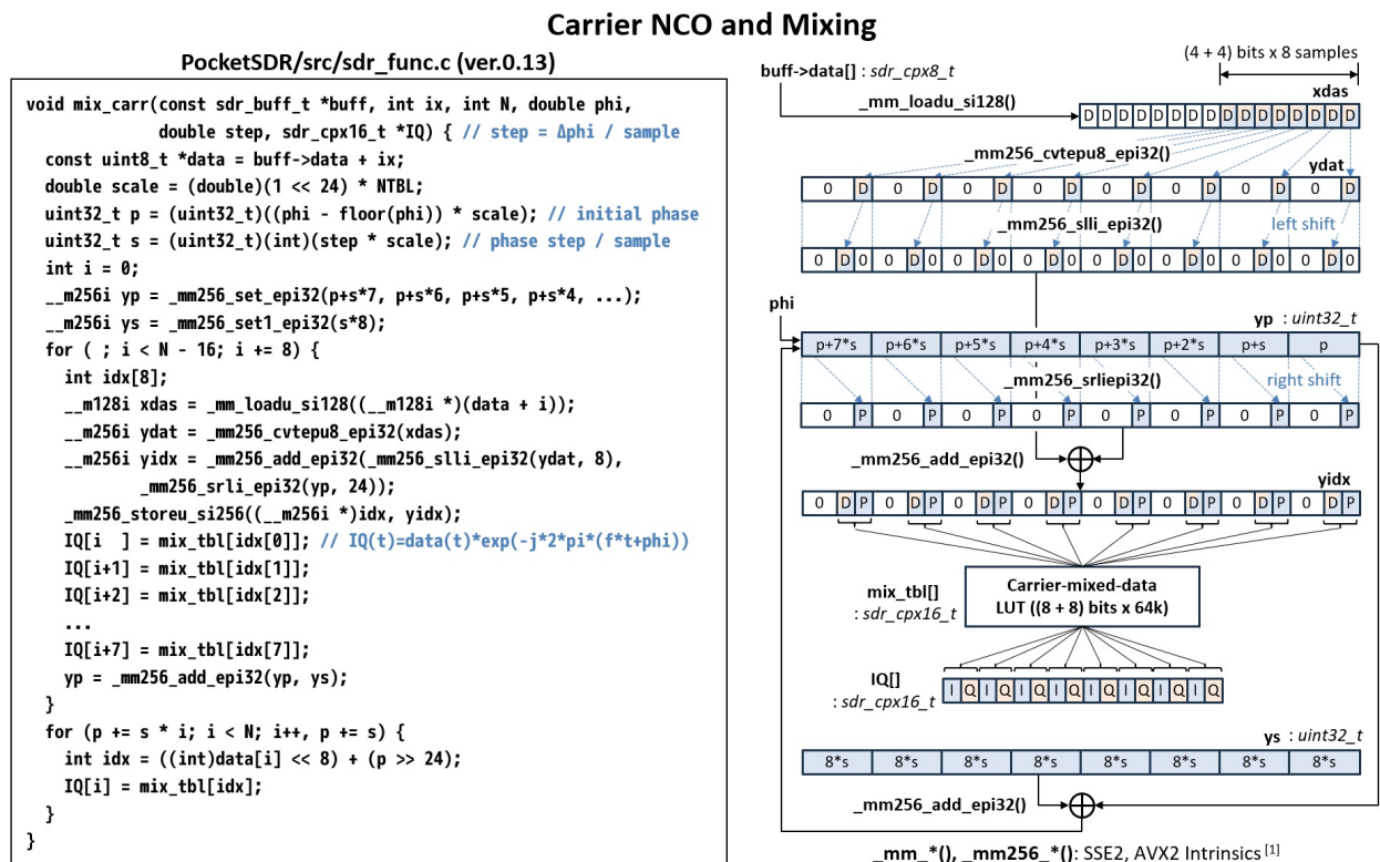
SIMD (AVX2) Optimization of Carrier Mixing
