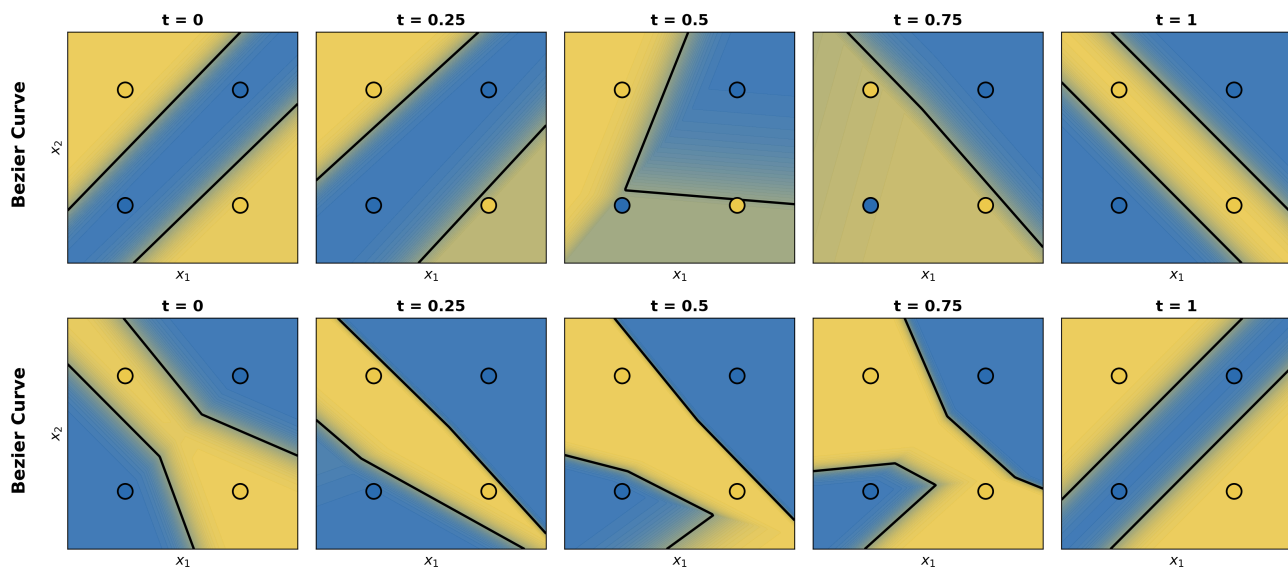
Figure 3: Nonlinear XOR paths. Top : a representative width-2 pair for which optimizing a Bézier path does not remove the high-loss region. Bottom : at width 3, a low-loss path connects endpoints with different decision boundaries. Rows visualize predictions along the learned path.
