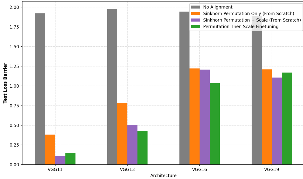
Figure 4: Maximum test-loss barrier for independently trained VGG models on CIFAR-10. Both scale-aware variants improve on Sinkhorn permutation-only for all four fixed endpoint pairs, although joint and sequential optimization trade places across architectures.
