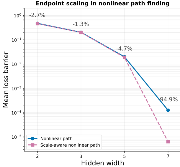
Figure 3: Mean nonlinear-path loss barrier by hidden width for polygonal paths with one interior control point, optimized from raw endpoints with or without independent positive scaling of both endpoints. Percentage annotations report the relative change under endpoint scaling; both curves aggregate the same endpoint pairs at each width.
