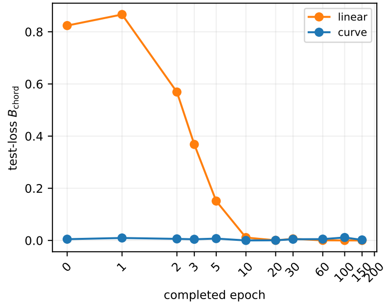
Within run: average of A_n \leftrightarrow A_{200} and B_n \leftrightarrow B_{200}
