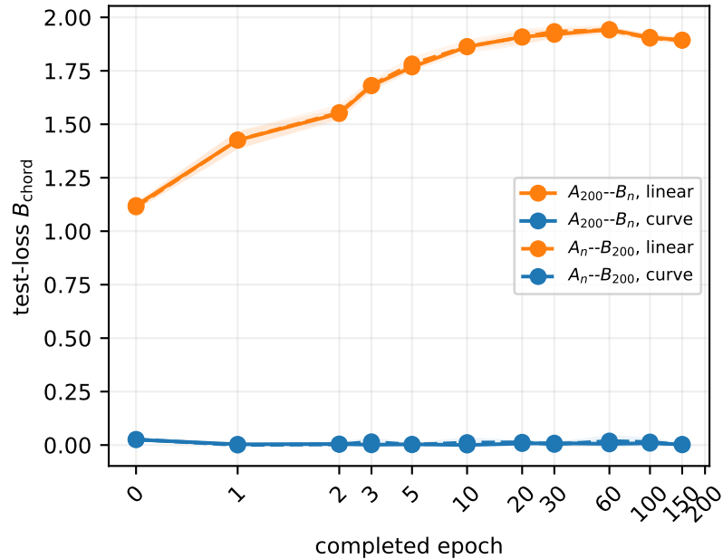
Independent models: cross stage
