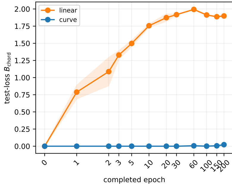
Independent models: A_n \leftrightarrow B_n
