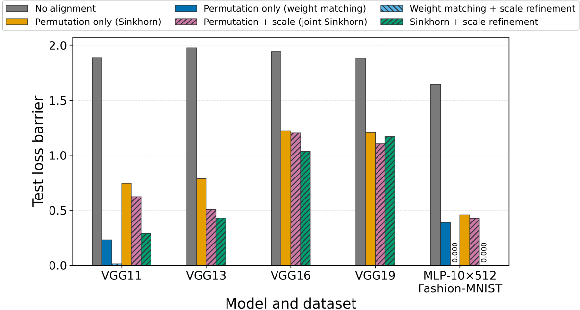
Figure 4: Test-loss barrier for independently trained VGG models on CIFAR-10 and a ten-layer width-512 MLP on Fashion-MNIST. Each group shows one fixed endpoint pair obtained from two independently trained runs. Weight matching and its scale refinement are available only for VGG11 and the MLP; absent bars denote methods that were not evaluated. Scale refinement improves both permutation methods wherever the corresponding baseline is available. The MLP uses a different alignment-fit protocol, so its absolute magnitude should not be compared directly with the VGG bars.
