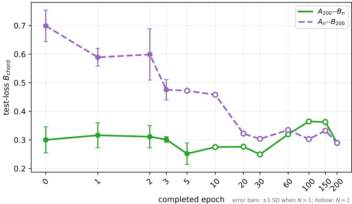
CIFAR-10 — VGG11 Sinkhorn + scale fine-tuning
