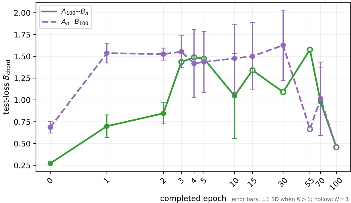
Fashion-MNIST — MLP 10×512 Sinkhorn permutation only
