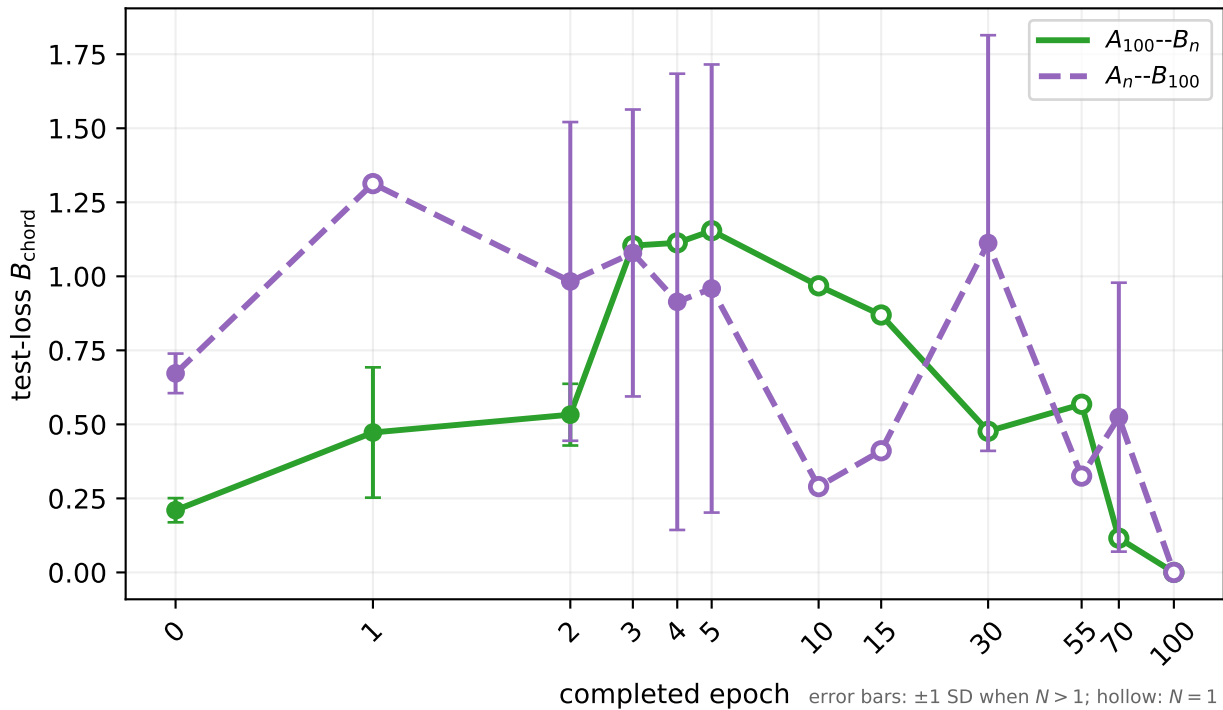
Fashion-MNIST — MLP 10×512 Sinkhorn + scale fine-tuning
