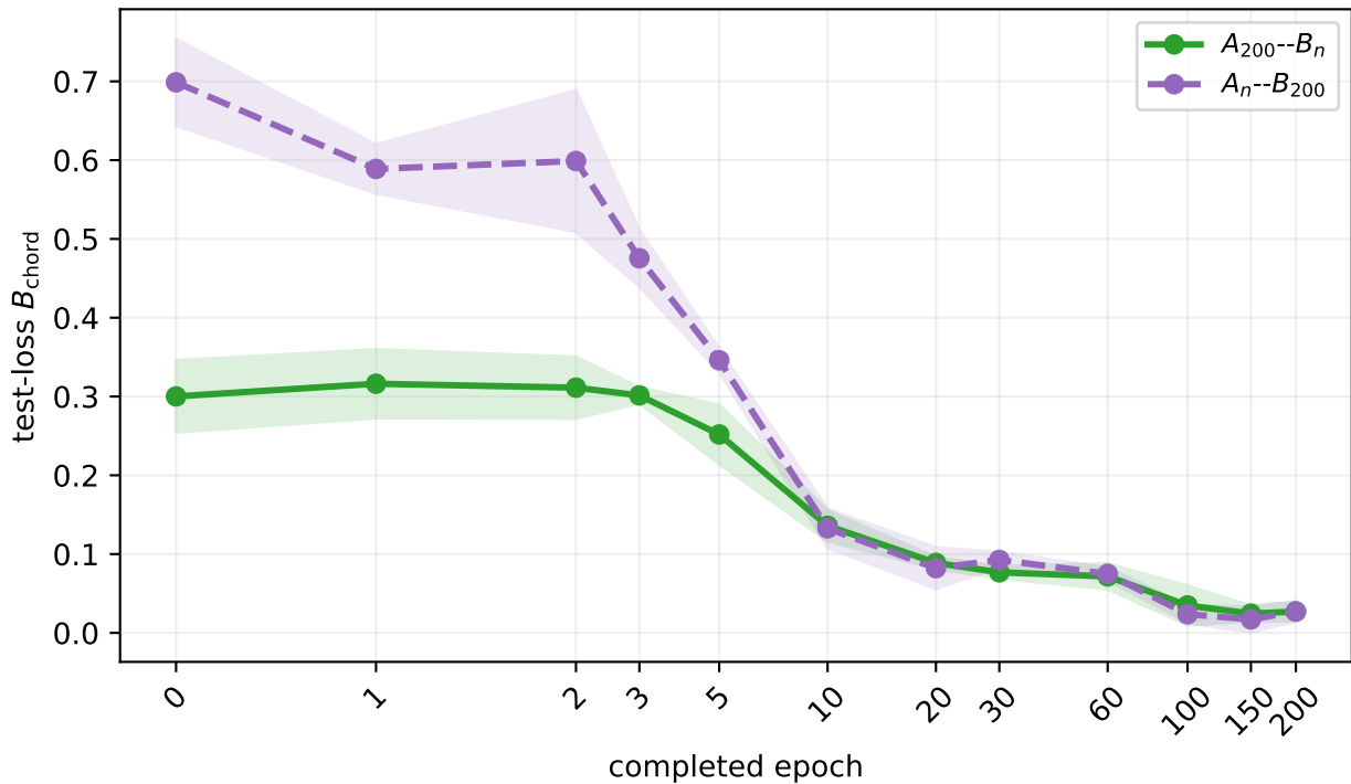
CIFAR-10 — VGG11 Best overall alignment
