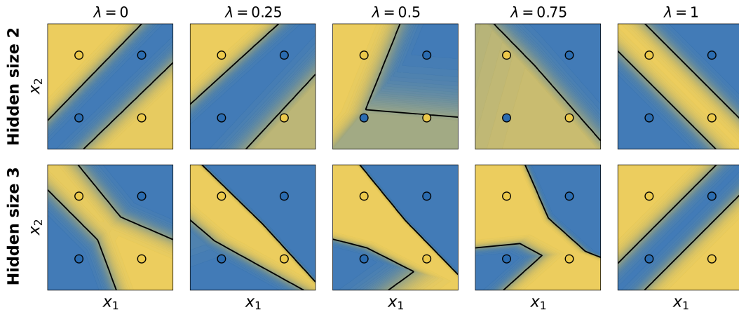
Figure A.1: Nonlinear XOR paths. Hidden size 2 : a representative pair for which optimizing a Bézier path does not remove the high-loss region. Hidden size 3 : a low-loss path connects endpoints with different decision boundaries. Rows visualize predictions along the learned path as a function of \lambda .
