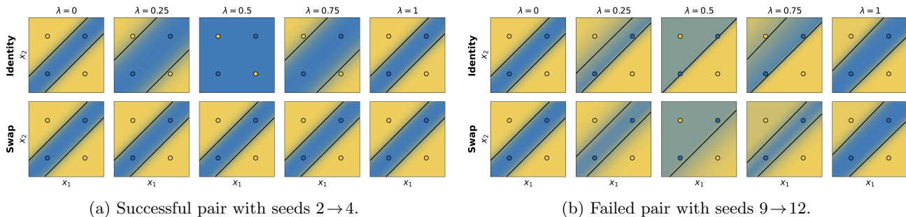
Figure 1: Decision boundaries along linear interpolation paths for two width-2 XOR endpoint pairs. Columns show interpolation values \lambda ; rows compare the identity and swap permutations.
