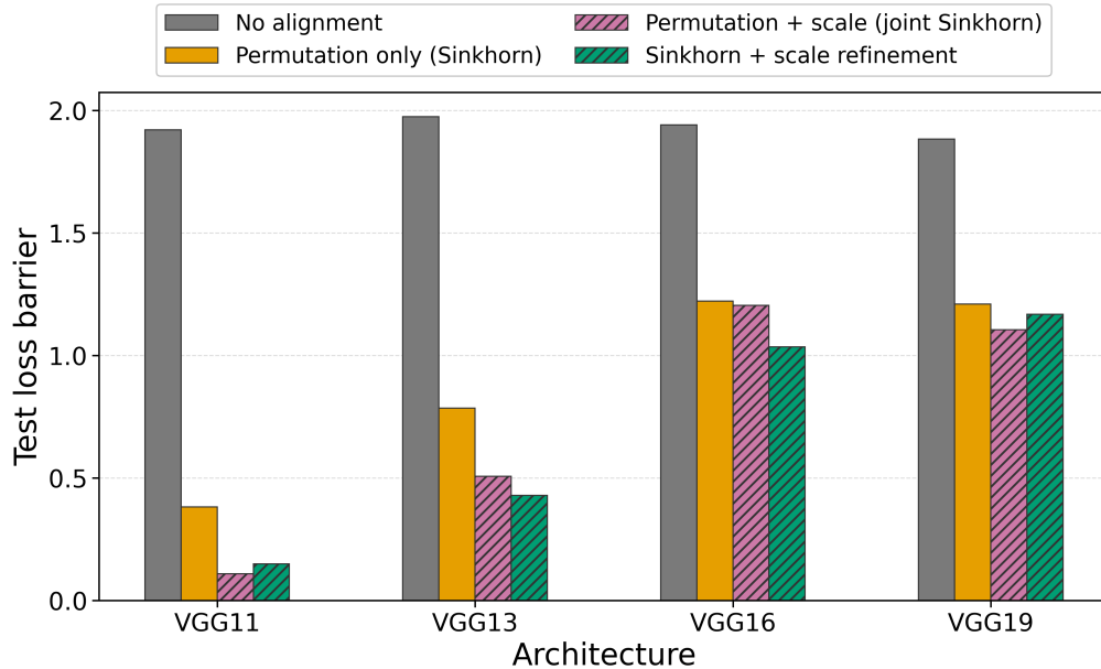
Figure 3: Maximum test-loss barrier for independently trained VGG models on CIFAR-10. Both scale-aware approaches improve on Sinkhorn permutation alignment for all four fixed endpoint pairs, although joint and sequential optimization trade places across architectures.
