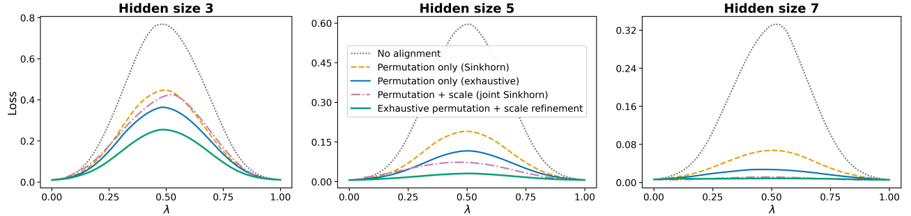
Figure A.2: Mean XOR interpolation-loss profiles at different hidden widths, comparing four alignment variants with raw interpolation. At each \lambda , loss is averaged across endpoint pairs.
