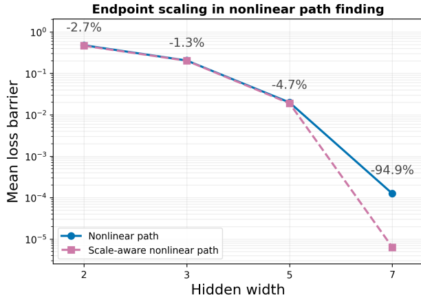
Figure 2: Mean nonlinear-path loss barrier by hidden width for polygonal paths with one interior control point, optimized from raw endpoints with or without independent positive scaling of both endpoints. Percentage annotations report the relative change under endpoint scaling.
