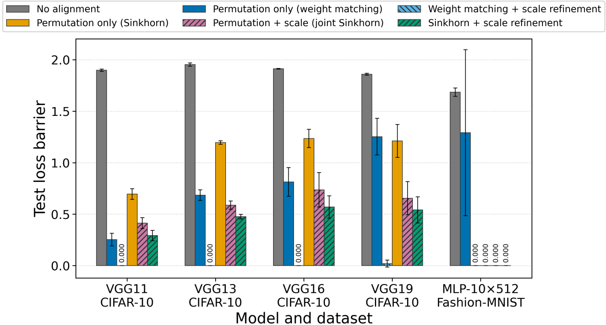
Figure 4: Test-loss barrier for independently trained VGG models on CIFAR-10 and a ten-layer width-512 MLP on Fashion-MNIST. Bars show the mean over three disjoint independently trained endpoint pairs, and error bars show the sample standard deviation. All six methods are evaluated for every architecture. Hyperparameters are selected separately for each pair using validation data only; barriers use the complete official test set after selections are frozen.
