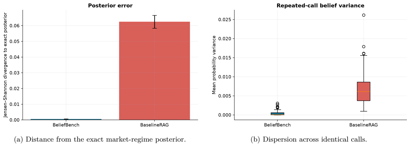
Figure 3: Financial case-study software diagnostics. The panels show whether the controlled pipeline preserves the exact posterior and whether repeated outputs are stable. They do not, by themselves, establish the quality of a frontier AI agent; that requires replacing the simulated adapter with a named OpenAI model and evaluating its absolute errors, calibration, elicited–inferred agreement, and decisions.
