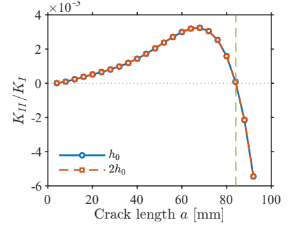
(d) Mode-mixity ratio K_{II}/K_I along the two independently propagated trajectories.
