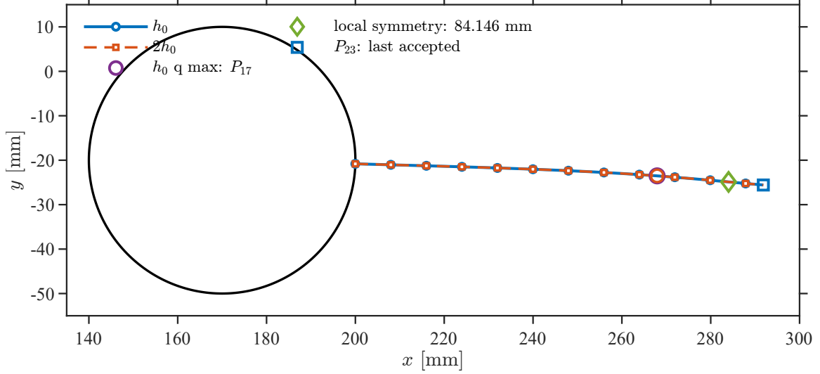
(a) Independently propagated trajectories for the production h_0 mesh family and the coarser 2h_0 structured core at fixed requested exterior sizing. The two paths are visually indistinguishable at the scale of the specimen.
