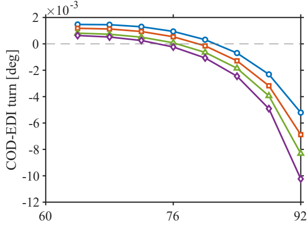
(a) Turning-angle differences for linear COD fits.
