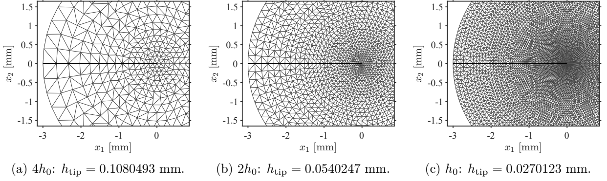
Figure 1: Structured near-tip mesh hierarchy at fixed core radius r_c = 3 mm, where h_0 = 0.0270123 mm is the production tip size. The panels use identical local coordinates and spatial limits. The 2h_0 and h_0 meshes satisfy the established native COD-sampling requirement. The 4h_0 mesh is included only to illustrate the geometric resolution hierarchy: its four COD windows contain 10, 15, 12, and 9 native points, so it is not admitted as a physically qualified mesh.
