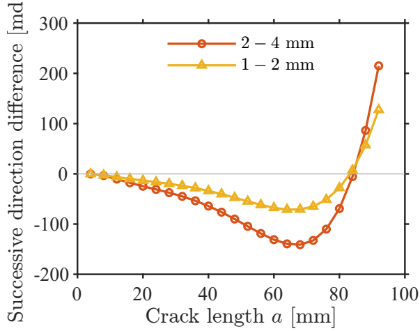
(c) Successive differences in absolute crack direction in the frozen initiation frame.
