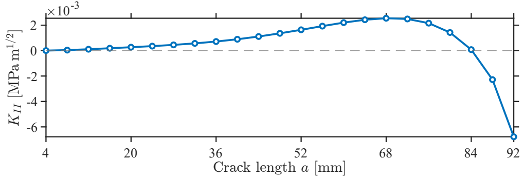
(b) Sliding-mode factor K_{II} .
