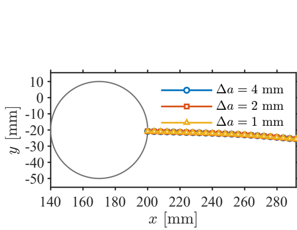
(a) Independently propagated crack trajectories for \Delta a = 4, 2 , and 1 mm, all continued to 92 mm.
