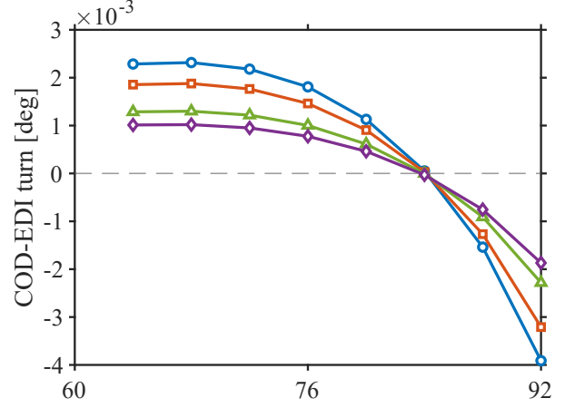
(b) Turning-angle differences for quadratic COD fits.
