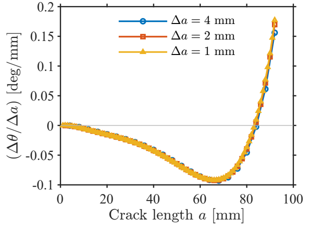
(d) Turning density \Delta\theta/\Delta a along the three independently propagated trajectories.
