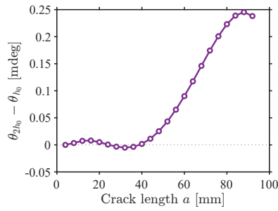
(c) Difference in the absolute crack direction in the frozen initiation frame, \theta_{2h_0} - \theta_{h_0} .
