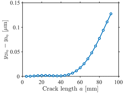
(b) Accumulated vertical tip-coordinate difference, y_{2h_0} - y_{h_0} .
