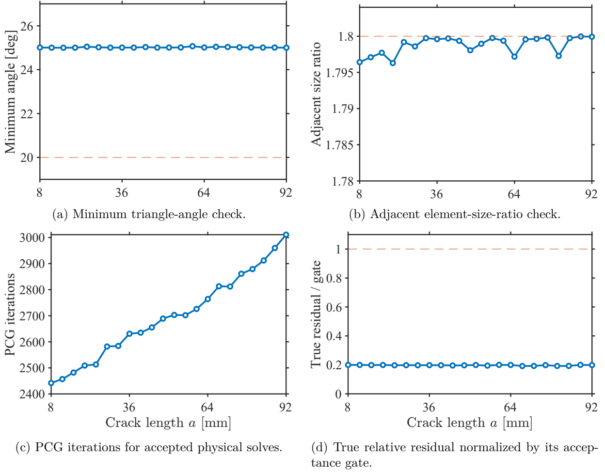
Figure S1: Diagnostics for accepted P_2 – P_{23} states. Dashed lines are the 20^\circ minimum-angle gate, 1.8 adjacent-size-ratio gate, and normalized true-residual gate of one. The separately enforced reported-PCG tolerance is 10^{-10} ; the true-residual acceptance denominator is 5 \times 10^{-10} . No failed P_{24} solve is plotted.
