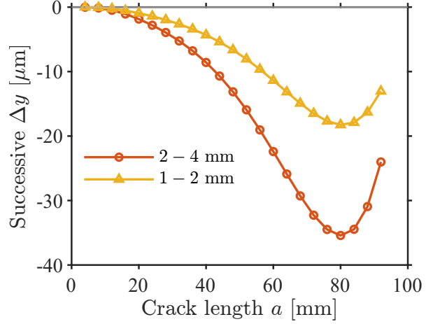
(b) Successive vertical-coordinate differences, y_{2\text{ mm}} - y_{4\text{ mm}} and y_{1\text{ mm}} - y_{2\text{ mm}} , evaluated at exact common crack lengths.
