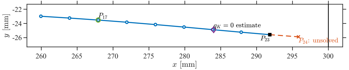
(b) Late-path detail with equal spatial scales. The markers identify P_{17} , the linearly interpolated K_{II}/K_I = 0 location, P_{23} , and the qualified unsolved point P_{24} .
