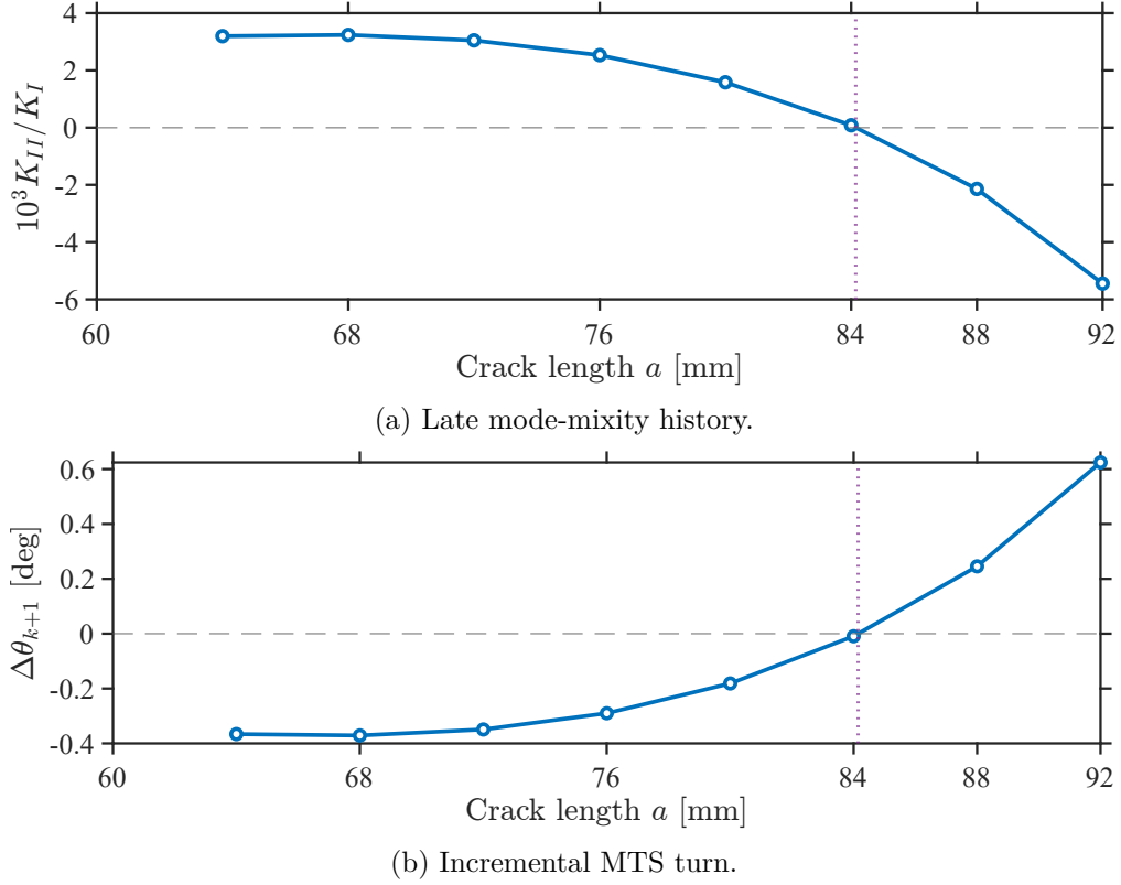
Figure 4: Mode-mixity sign reversal and opposite-signed MTS turning. Each marker is an accepted current-tip state; its turn predicts the next segment. The vertical dotted line is the interpolated K_{II}/K_I = 0 location. The positive turn reported at a = 92 mm belongs to the P_{23} solution and predicts the unsolved next geometry.
