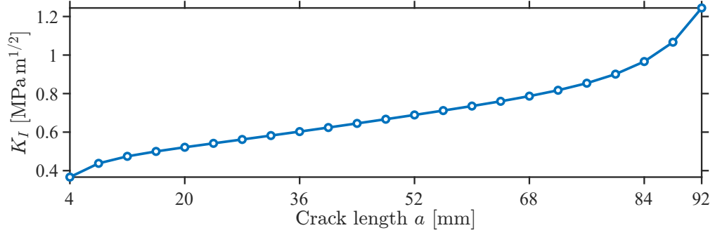
(a) Opening-mode factor K_I .
