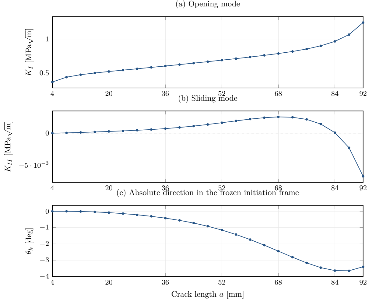
Figure 2: Accepted intensities and absolute direction. Intensities correspond to unit remote traction. The direction minimum occurs at P_{22} ; positive turning there produces the less negative P_{23} direction. No physical curve includes P_{24} .
