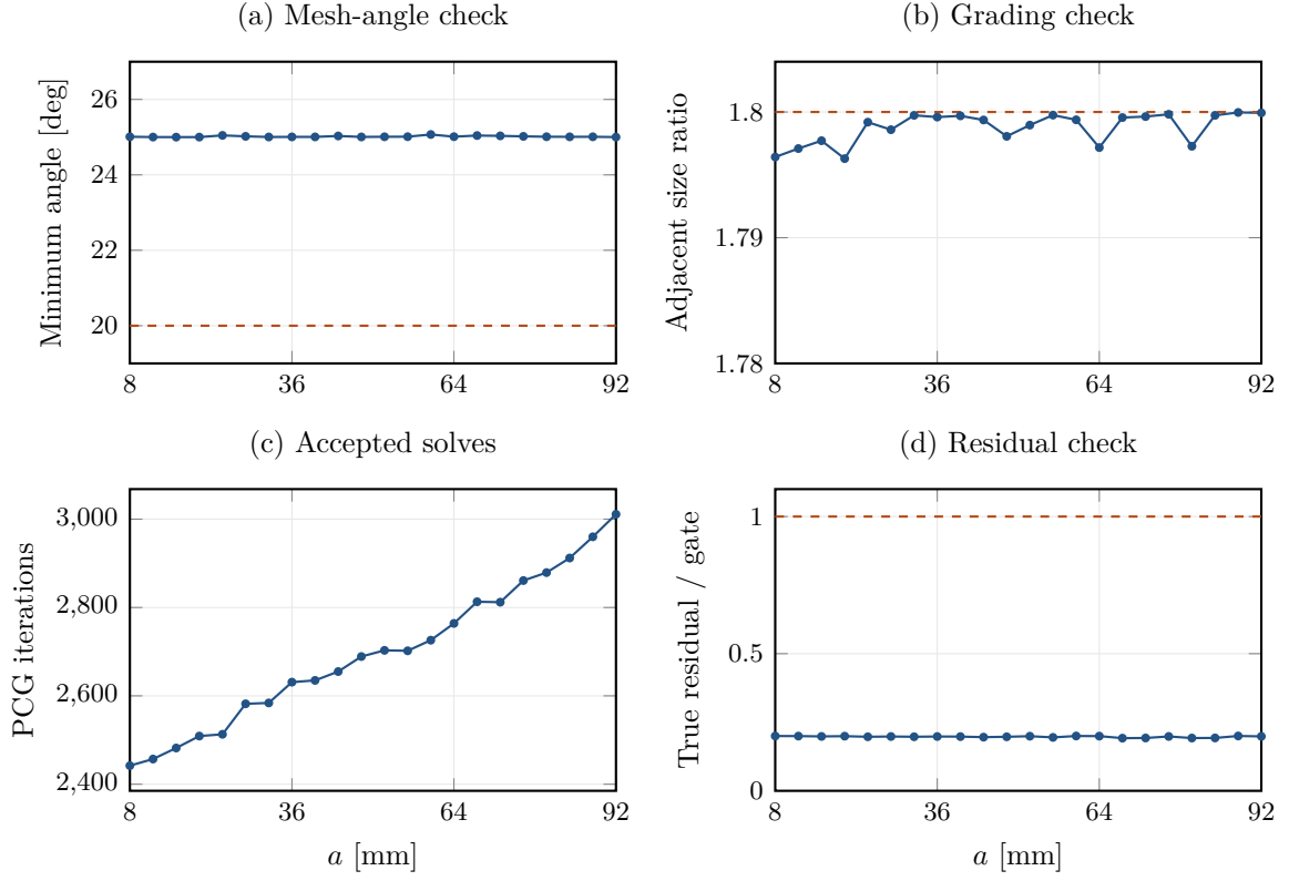
Figure S1: Diagnostics for accepted P_2 – P_{23} states. Dashed lines are the 20^\circ minimum-angle gate, 1.8 adjacent-size-ratio gate, and normalized true-residual gate of one. The separately enforced reported-PCG tolerance is 10^{-10} ; the true-residual acceptance denominator is 5 \times 10^{-10} . No failed P_{24} solve is plotted.
