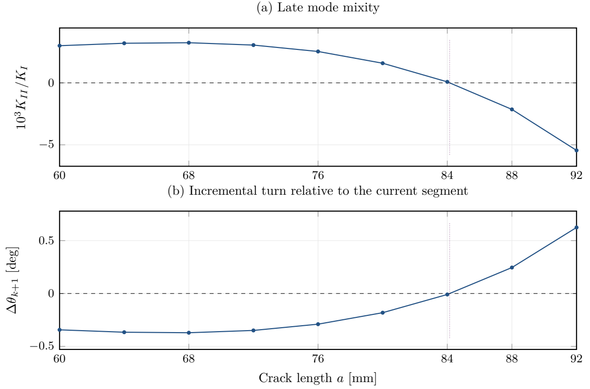
Figure 3: Mode-mixity sign reversal and opposite-signed MTS turning. Each marker is an accepted current-tip state; its turn predicts the next segment. The vertical dotted line is the interpolated q_K = 0 location. The positive turn reported at a = 92 mm belongs to the P_{23} solution and predicts the unsolved next geometry.
