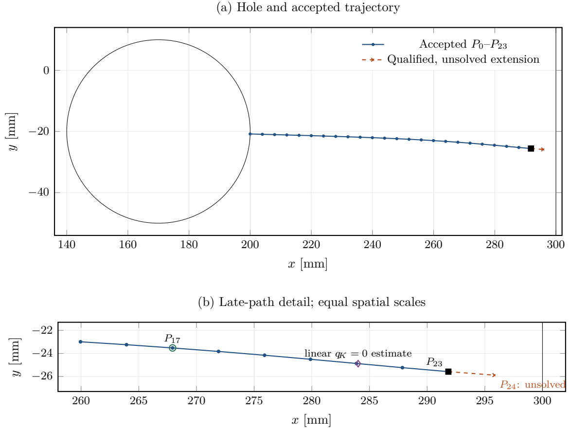
Figure 1: Hole-initiated trajectory and late detail. Both spatial panels use equal x and y scales within the panel. The circle gives geometric context; the numerical hole is polygonally discretized. Solid segments are accepted geometry through P_{23} . The dashed extension is qualified geometry only and has no accepted physical SIFs. The diamond is a linear interpolation marker, not a solved tip.
