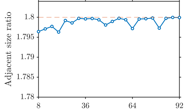
(b) Adjacent element-size-ratio check.
