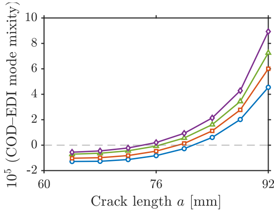
(c) Mode-mixity differences for linear COD fits.
