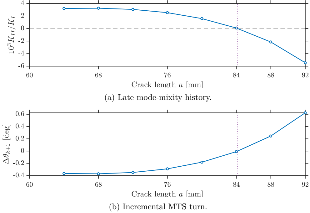
Figure 5: Mode-mixity sign reversal and opposite-signed MTS turning. Each marker is an accepted current-tip state; its turn predicts the next segment. The vertical dotted line is the interpolated K_{II}/K_I = 0 location. The positive turn reported at a = 92 mm belongs to the P_{23} solution and predicts the unsolved next geometry.
