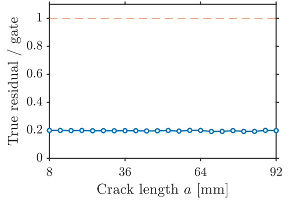
(d) True relative residual normalized by its acceptance gate.
