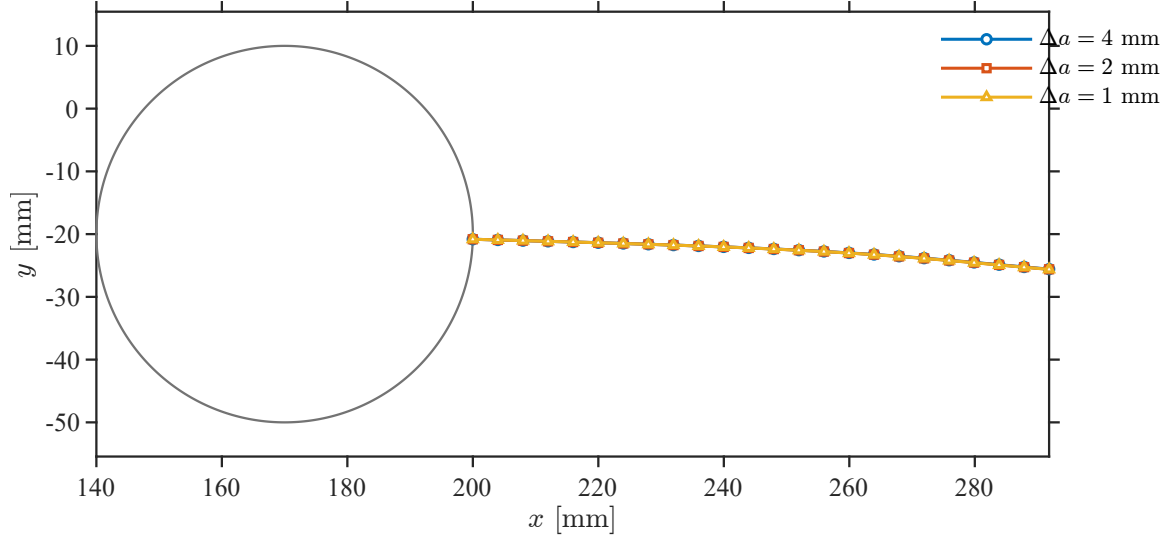
(a) Independently propagated crack trajectories for \Delta a = 4, 2 , and 1 mm, all continued to 92 mm.
