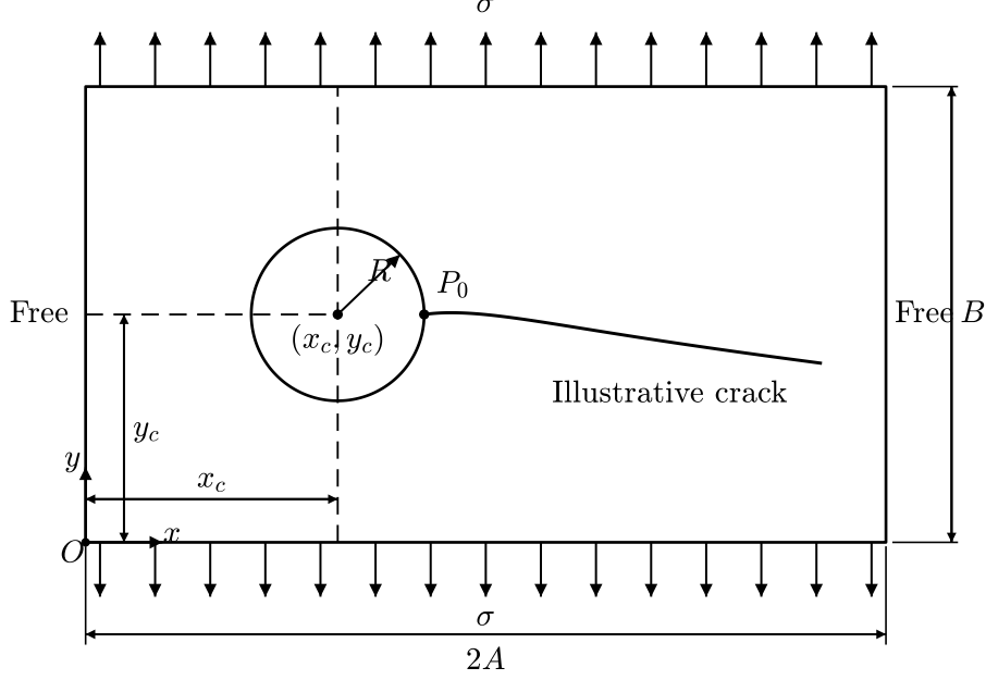
Figure 1: Specimen geometry and tensile loading. The plate has width 2A and height B , and the circular hole has radius R and center (x_c, y_c) in the schematic's lower-left coordinate system. The computational y coordinate is shifted by -B/2 relative to the sketch. The symbolic sketch is not drawn to the numerical scale. The arrows indicate outward tensile tractions of unsigned magnitude \sigma ; the lateral edges, hole boundary, and crack faces are traction-free. The curvilinear crack is schematic, not a prescribed or independently solved trajectory.
