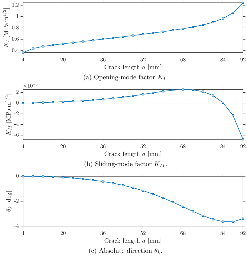
Figure 4: Accepted intensities and absolute direction in the frozen initiation frame. Intensities correspond to unit remote traction. The direction minimum occurs at P_{22} ; positive turning there produces the less negative P_{23} direction. No physical curve includes P_{24} .
