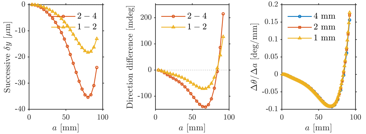
(b) Successive vertical-coordinate differences, y_{2\text{ mm}} - y_{4\text{ mm}} and y_{1\text{ mm}} - y_{2\text{ mm}} , evaluated at exact common crack lengths.
