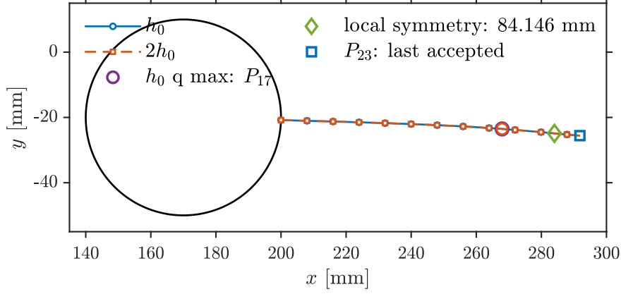
(a) Independently propagated trajectories for the production h_0 mesh family and the coarser 2h_0 structured core at fixed requested exterior sizing. The two paths are visually indistinguishable at the scale of the specimen.
