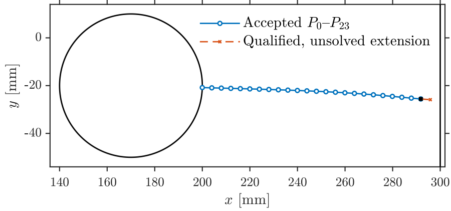
(a) Hole and accepted trajectory through P_{23} , with the qualified but physically unsolved P_{23} – P_{24} extension.
