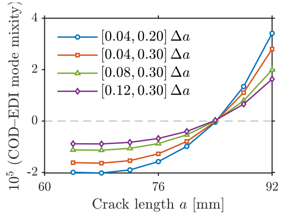
(d) Mode-mixity differences for quadratic COD fits.
