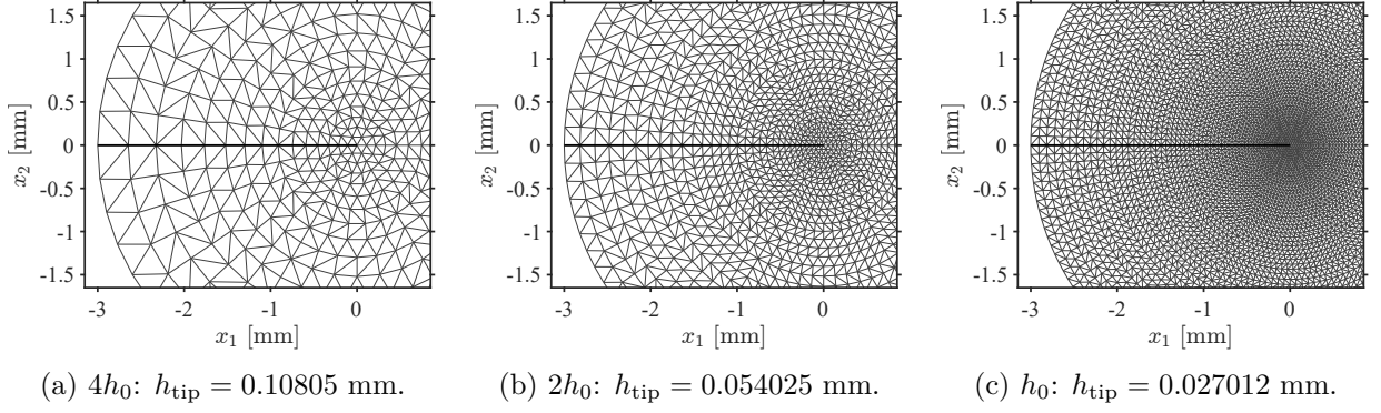
Figure 2: Structured near-tip mesh hierarchy at fixed core radius r_c = 3 mm, where h_0 = 0.027012 mm is the production tip size. The panels use identical local coordinates and spatial limits. The 2h_0 and h_0 meshes satisfy the established native COD-sampling requirement. The 4h_0 mesh is included only to illustrate the geometric resolution hierarchy: its four COD windows contain 10, 15, 12, and 9 native points, so it is not admitted as a physically qualified mesh.
