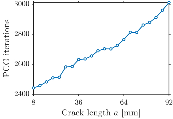
(c) PCG iterations for accepted physical solves.
