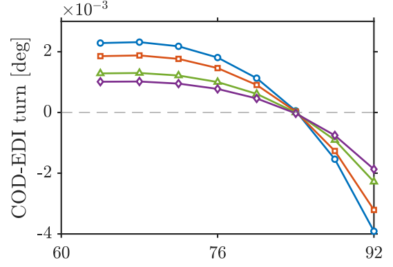
(b) Turning-angle differences for quadratic COD fits.
