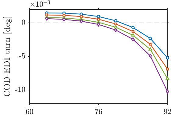
(a) Turning-angle differences for linear COD fits.
