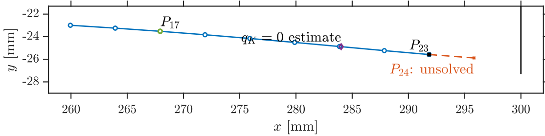
(b) Late-path detail with equal spatial scales. The markers identify P_{17} , the linearly interpolated K_{II}/K_I = 0 location, P_{23} , and the qualified unsolved point P_{24} .
