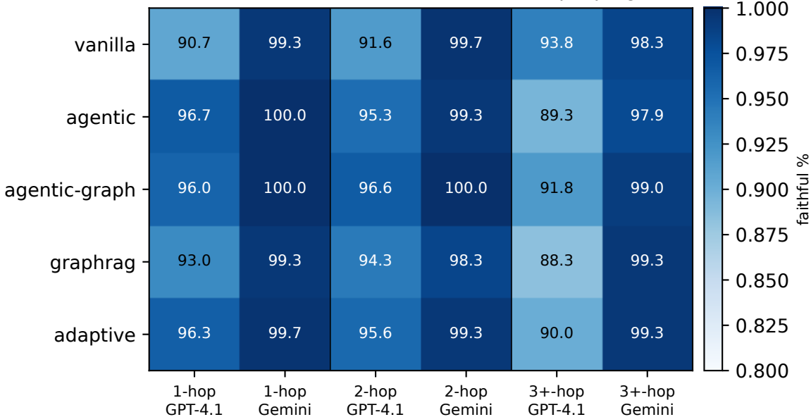
Faithfulness % (full v2 matrix, n=4,440 per judge)
