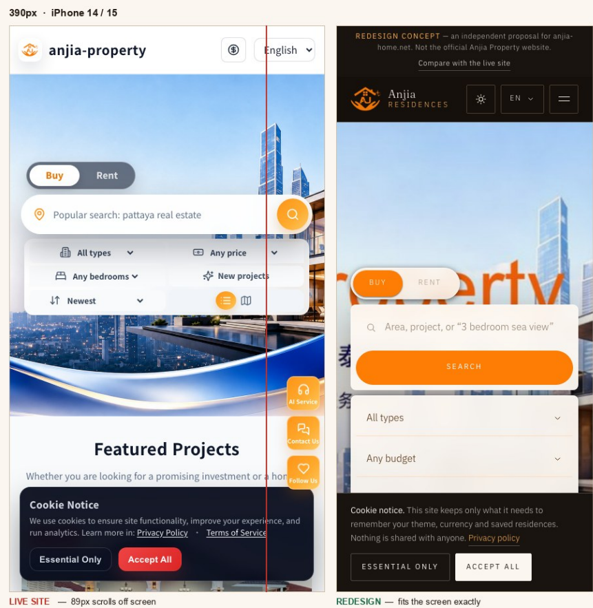
The homepage today (left) and the source-faithful warm proposal (right) on an iPhone 14. The screenshots are unretouched layout evidence from the refreshed build, which contains the verified 169-record source set.
