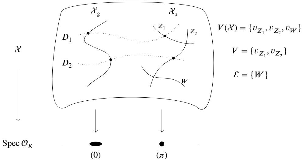
Figure 1.1: Illustration of the proof of Proposition 1.29 (ii)
